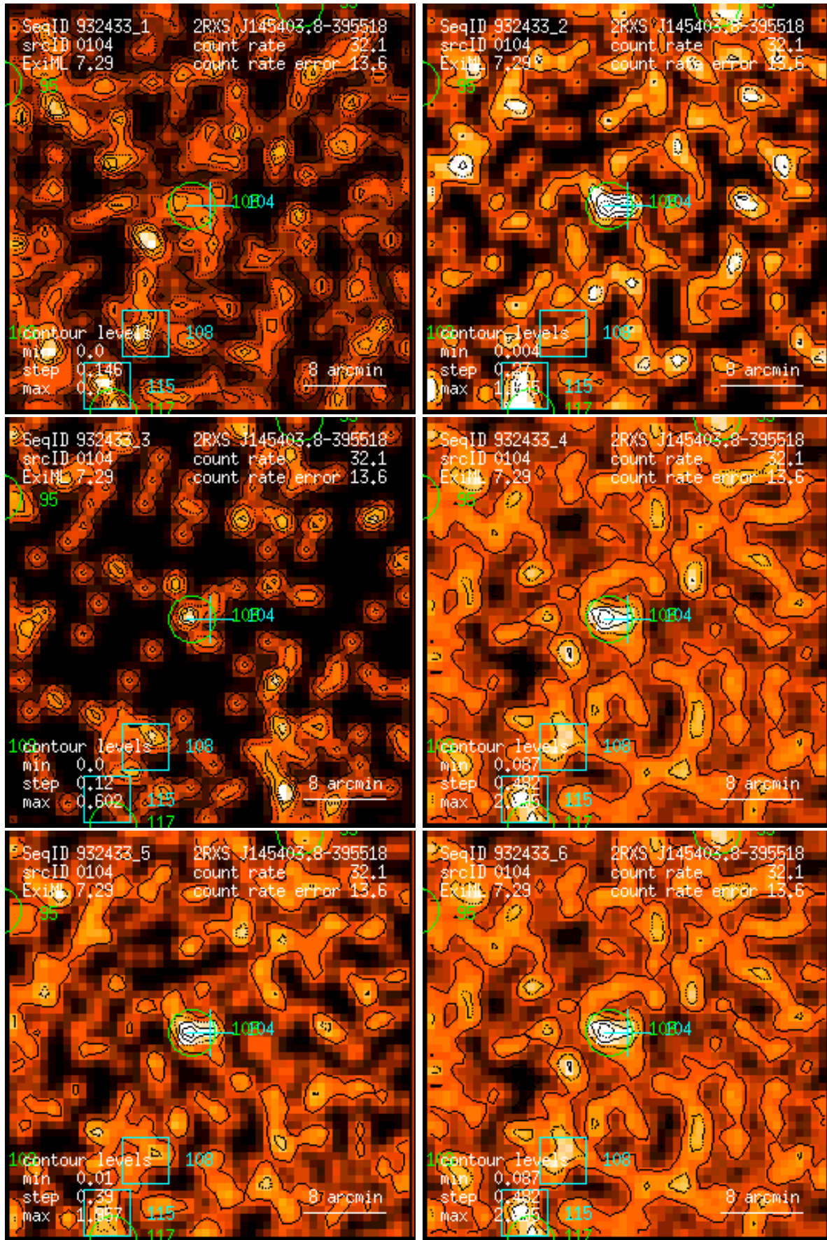
Figure 104: RASS 932433: detection 0104: band rate images, Gaussian filter: (1) PSPC channels 11 – 41, (2) 52 – 90, (3) 91 – 201, (4) 11 – 235, (5) 52 – 201, (6) 11 – 201. Broad band rates in counts/ks. Band rate contour levels in counts/ks/arcmin 2 .
