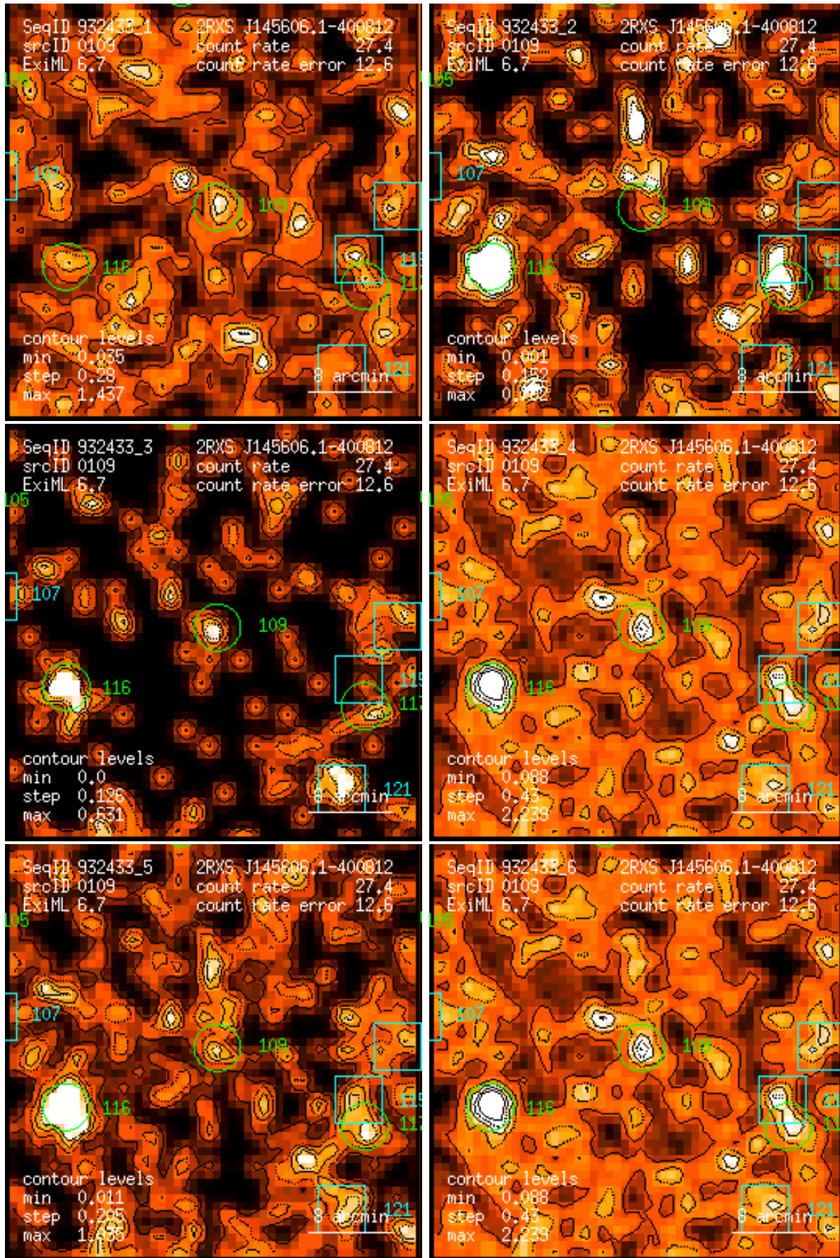
Figure 109: RASS 932433: detection 0109: band rate images, Gaussian filter: (1) PSPC channels 11 – 41, (2) 52 – 90, (3) 91 – 201, (4) 11 – 235, (5) 52 – 201, (6) 11 – 201. Broad band rates in counts/ks. Band rate contour levels in counts/ks/arcmin 2 .
