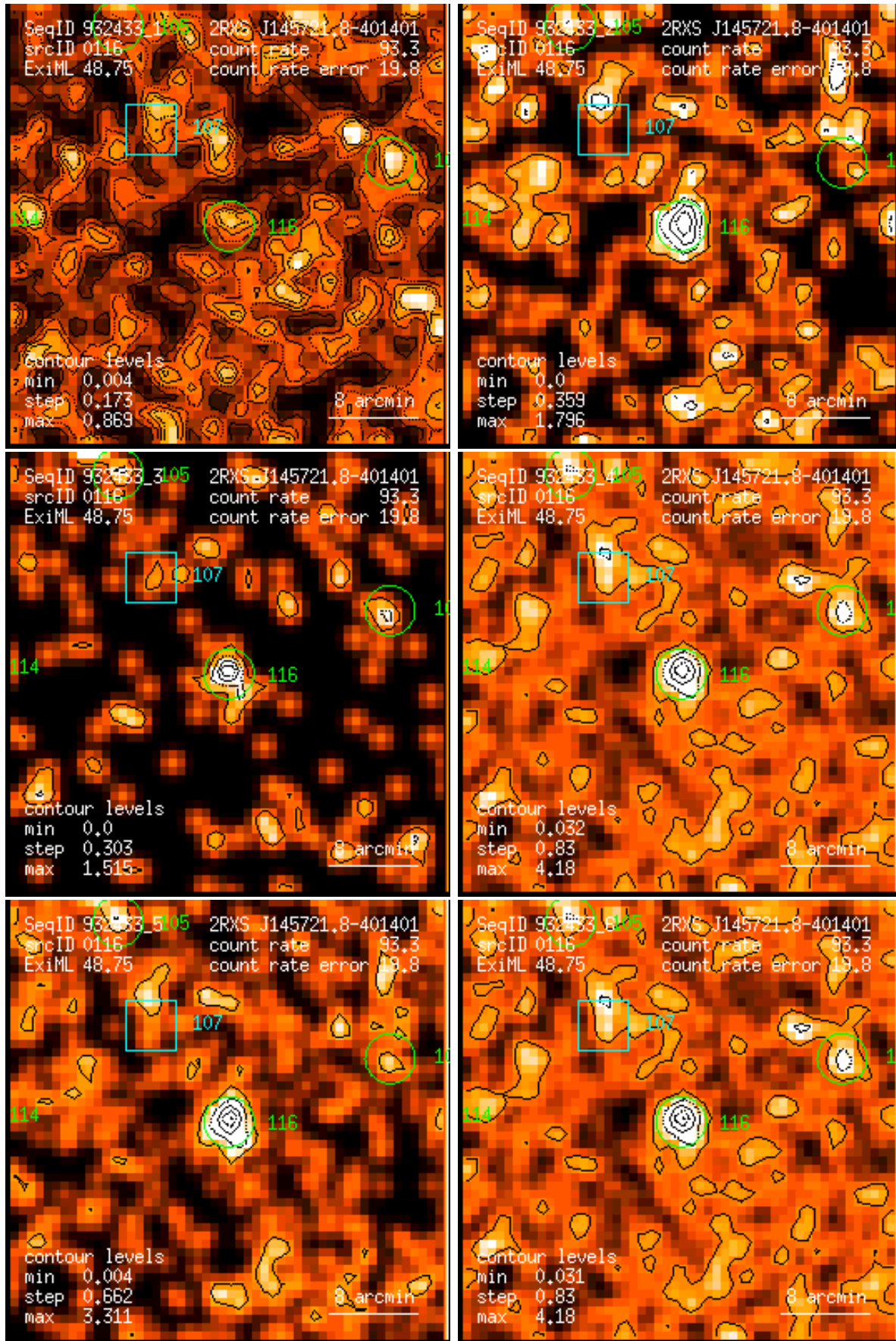
Figure 116: RASS 932433: detection 0116: band rate images, Gaussian filter: (1) PSPC channels 11 – 41, (2) 52 – 90, (3) 91 – 201, (4) 11 – 235, (5) 52 – 201, (6) 11 – 201. Broad band rates in counts/ks. Band rate contour levels in counts/ks/arcmin 2 .
