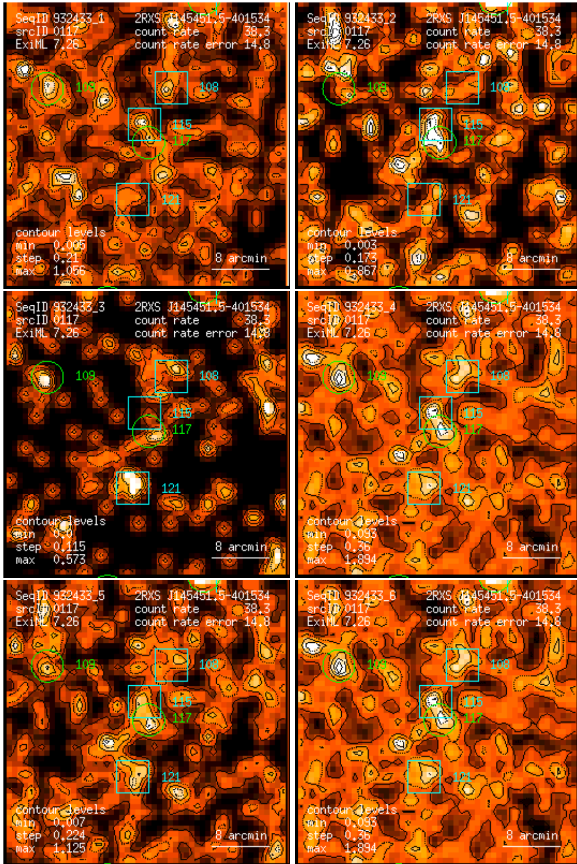
Figure 117: RASS 932433: detection 0117: band rate images, Gaussian filter: (1) PSPC channels 11 – 41, (2) 52 – 90, (3) 91 – 201, (4) 11 – 235, (5) 52 – 201, (6) 11 – 201. Broad band rates in counts/ks. Band rate contour levels in counts/ks/arcmin 2 .
