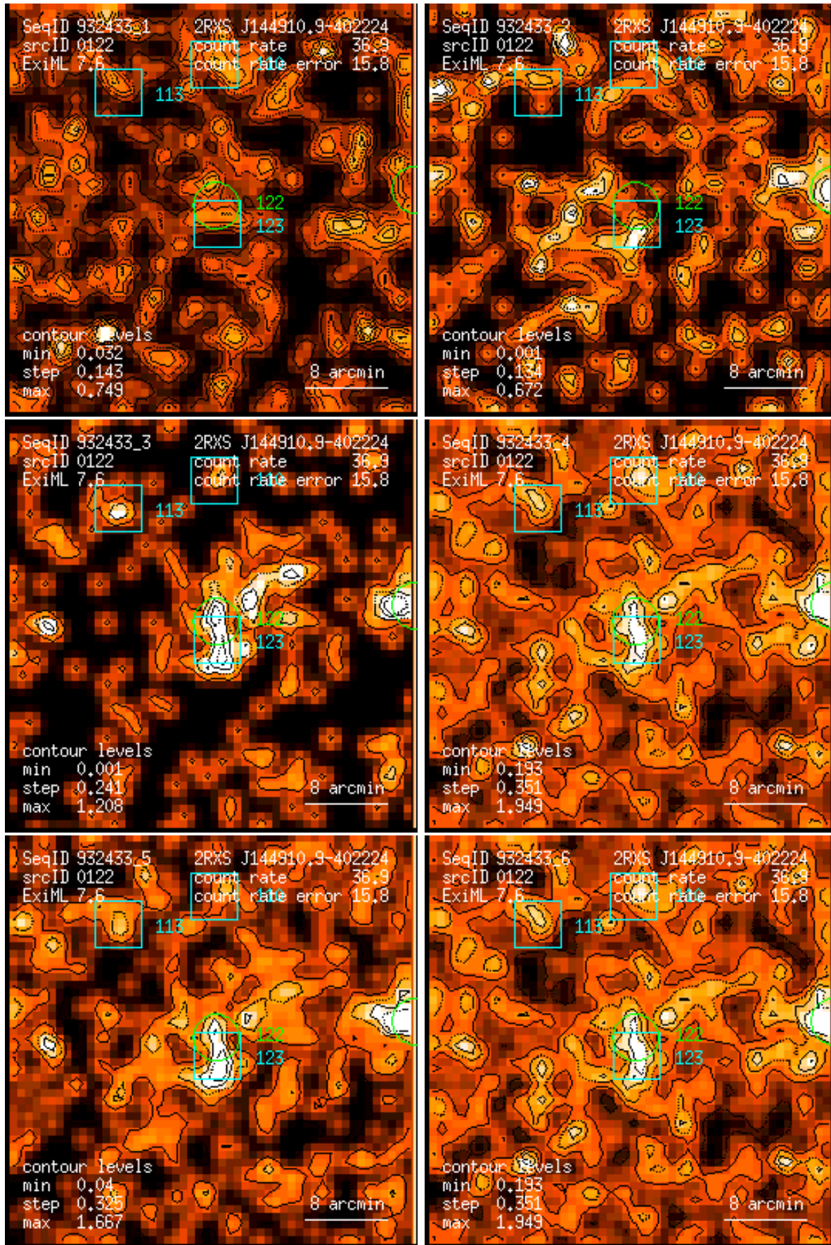
Figure 122: RASS 932433: detection 0122: band rate images, Gaussian filter: (1) PSPC channels 11 – 41, (2) 52 – 90, (3) 91 – 201, (4) 11 – 235, (5) 52 – 201, (6) 11 – 201. Broad band rates in counts/ks. Band rate contour levels in counts/ks/arcmin 2 .
