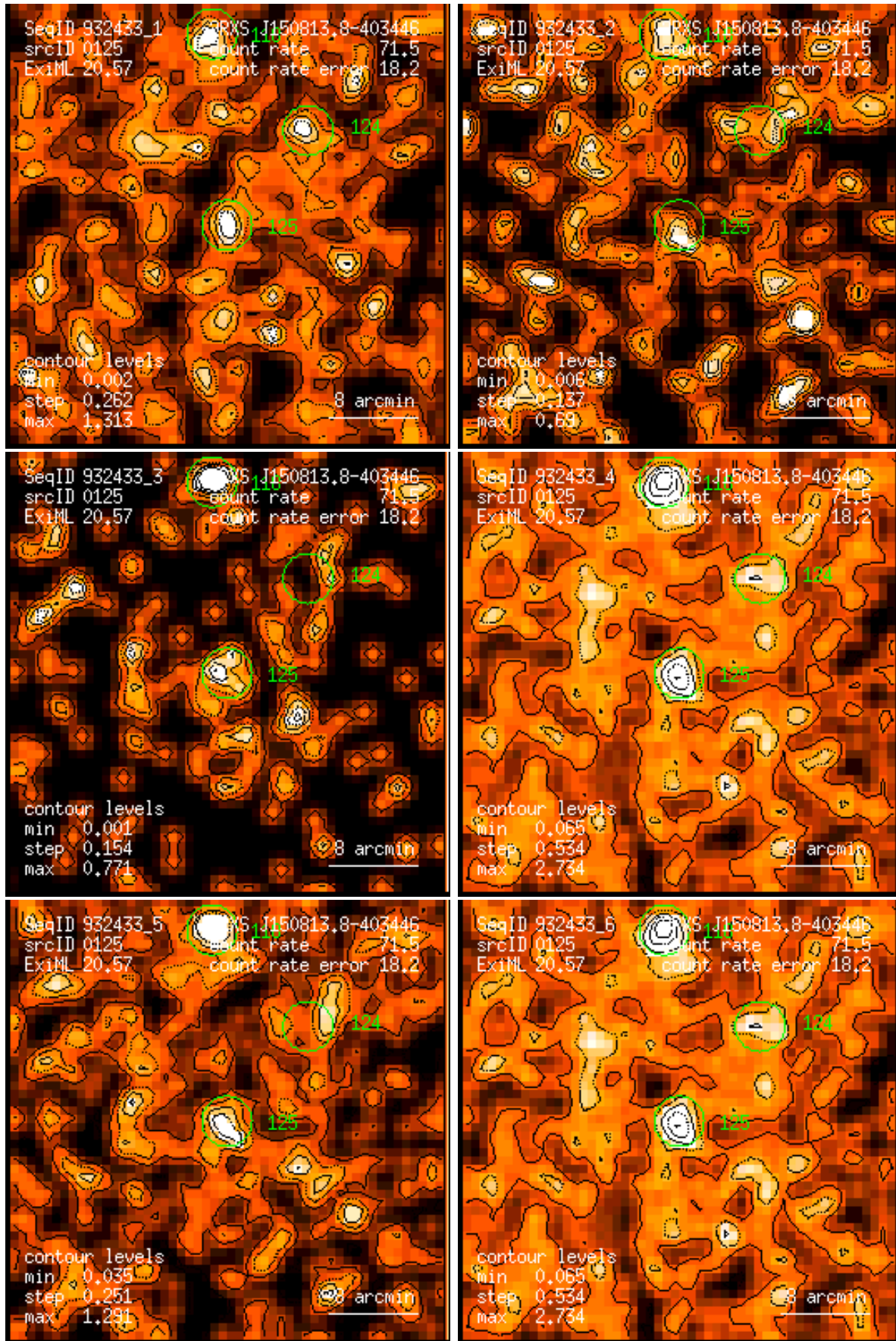
Figure 125: RASS 932433: detection 0125: band rate images, Gaussian filter: (1) PSPC channels 11 – 41, (2) 52 – 90, (3) 91 – 201, (4) 11 – 235, (5) 52 – 201, (6) 11 – 201. Broad band rates in counts/ks. Band rate contour levels in counts/ks/arcmin 2 .
