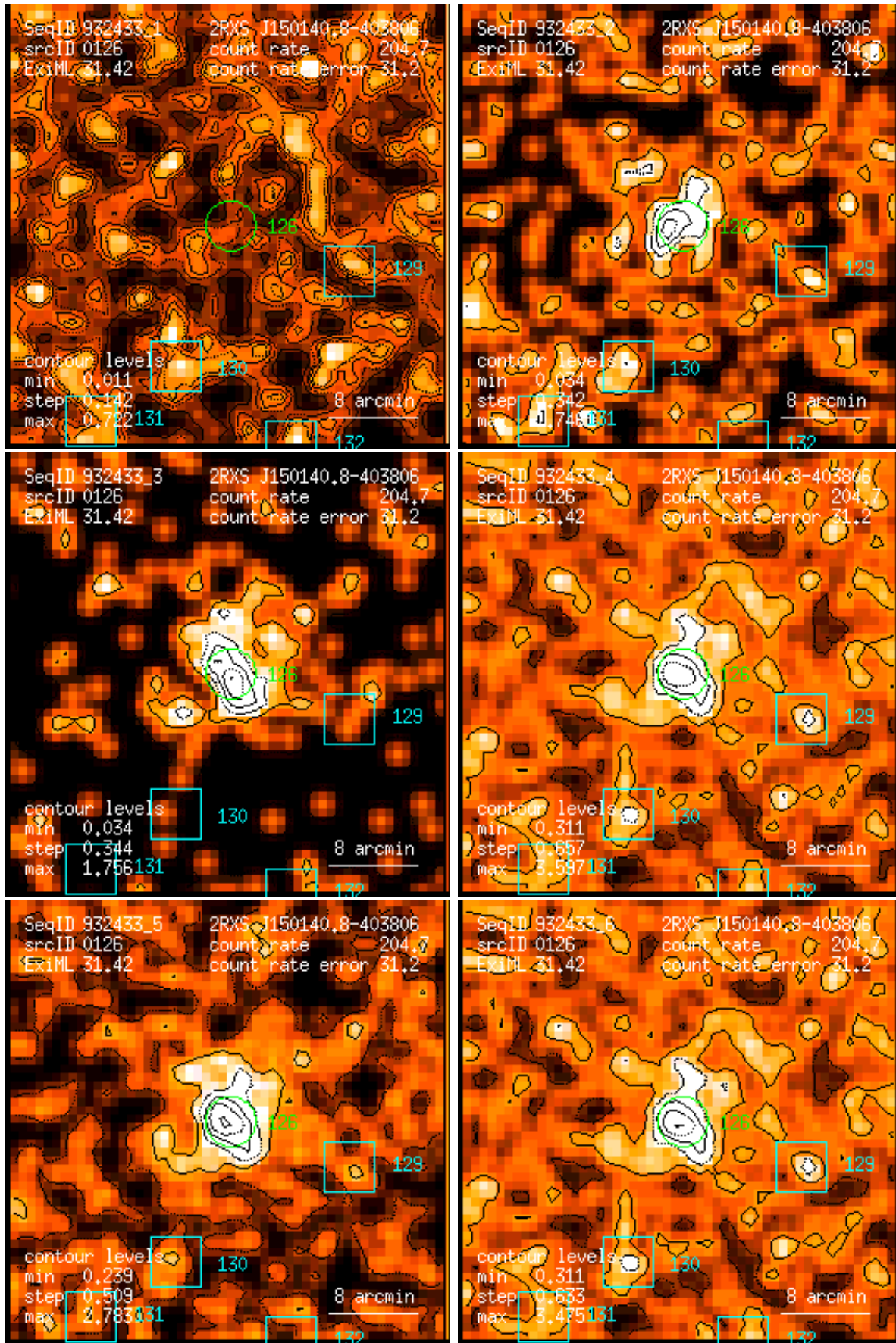
Figure 126: RASS 932433: detection 0126: band rate images, Gaussian filter: (1) PSPC channels 11 – 41, (2) 52 – 90, (3) 91 – 201, (4) 11 – 235, (5) 52 – 201, (6) 11 – 201. Broad band rates in counts/ks. Band rate contour levels in counts/ks/arcmin 2 .
