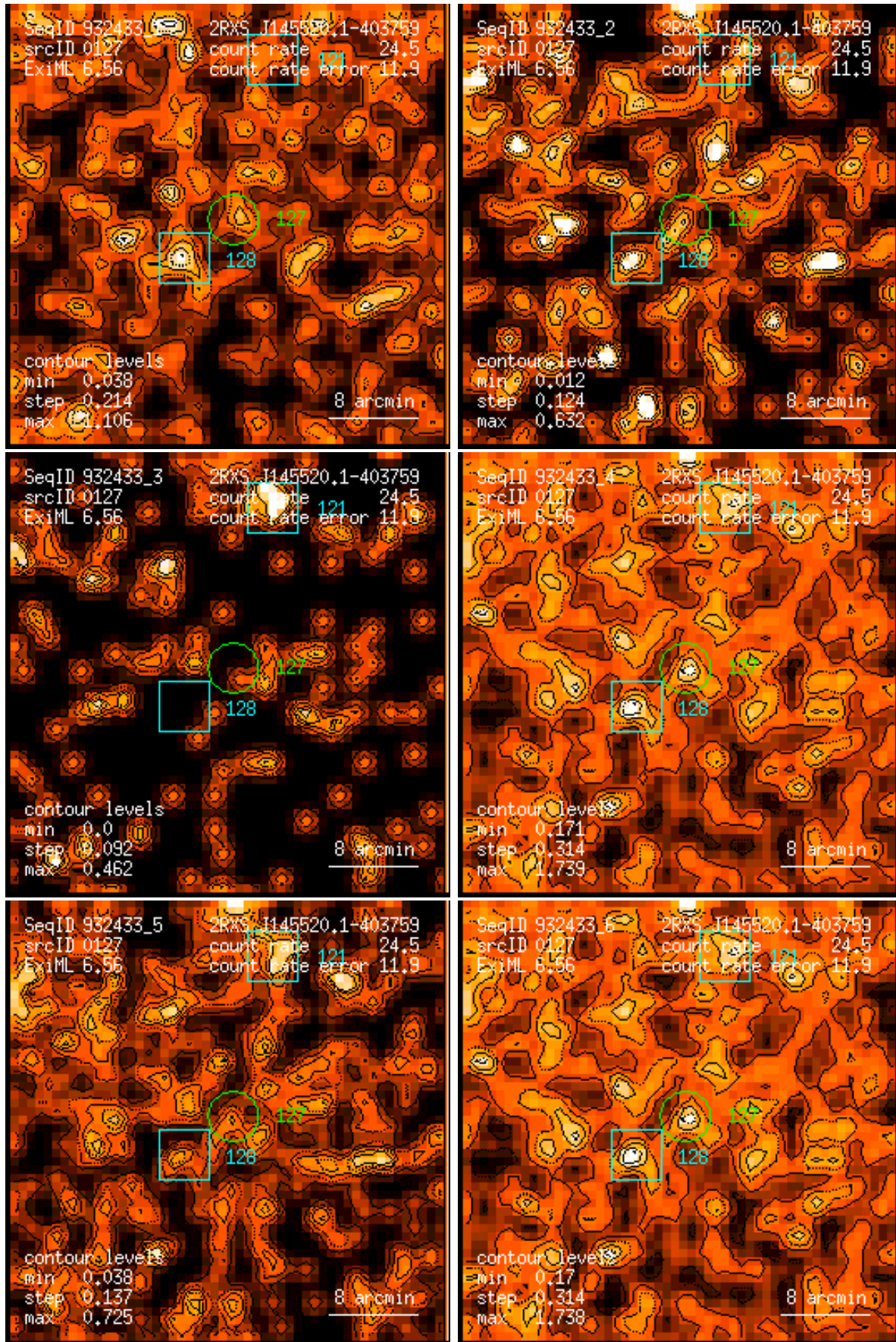
Figure 127: RASS 932433: detection 0127: band rate images, Gaussian filter: (1) PSPC channels 11 – 41, (2) 52 – 90, (3) 91 – 201, (4) 11 – 235, (5) 52 – 201, (6) 11 – 201. Broad band rates in counts/ks. Band rate contour levels in counts/ks/arcmin 2 .
