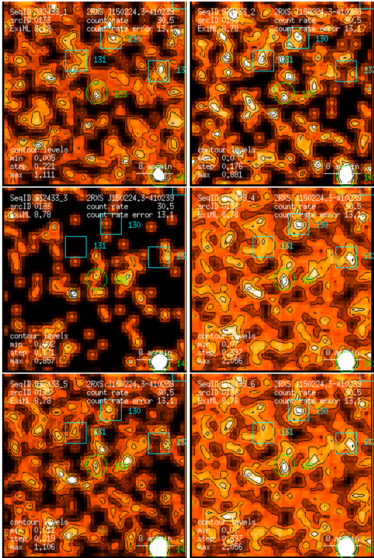
Figure 133: RASS 932433: detection 0133: band rate images, Gaussian filter: (1) PSPC channels 11 – 41, (2) 52 – 90, (3) 91 – 201, (4) 11 – 235, (5) 52 – 201, (6) 11 – 201. Broad band rates in counts/ks. Band rate contour levels in counts/ks/arcmin 2 .
