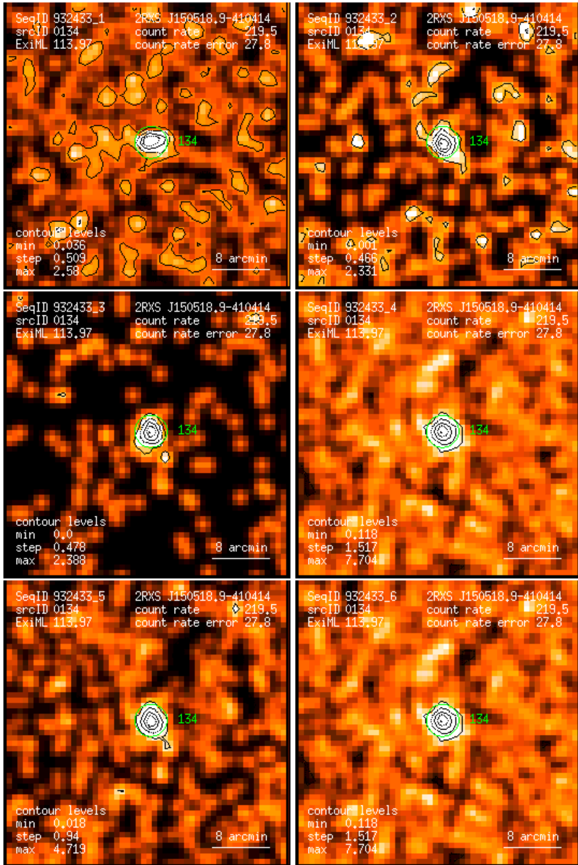
Figure 134: RASS 932433: detection 0134: band rate images, Gaussian filter: (1) PSPC channels 11 – 41, (2) 52 – 90, (3) 91 – 201, (4) 11 – 235, (5) 52 – 201, (6) 11 – 201. Broad band rates in counts/ks. Band rate contour levels in counts/ks/arcmin 2 .
