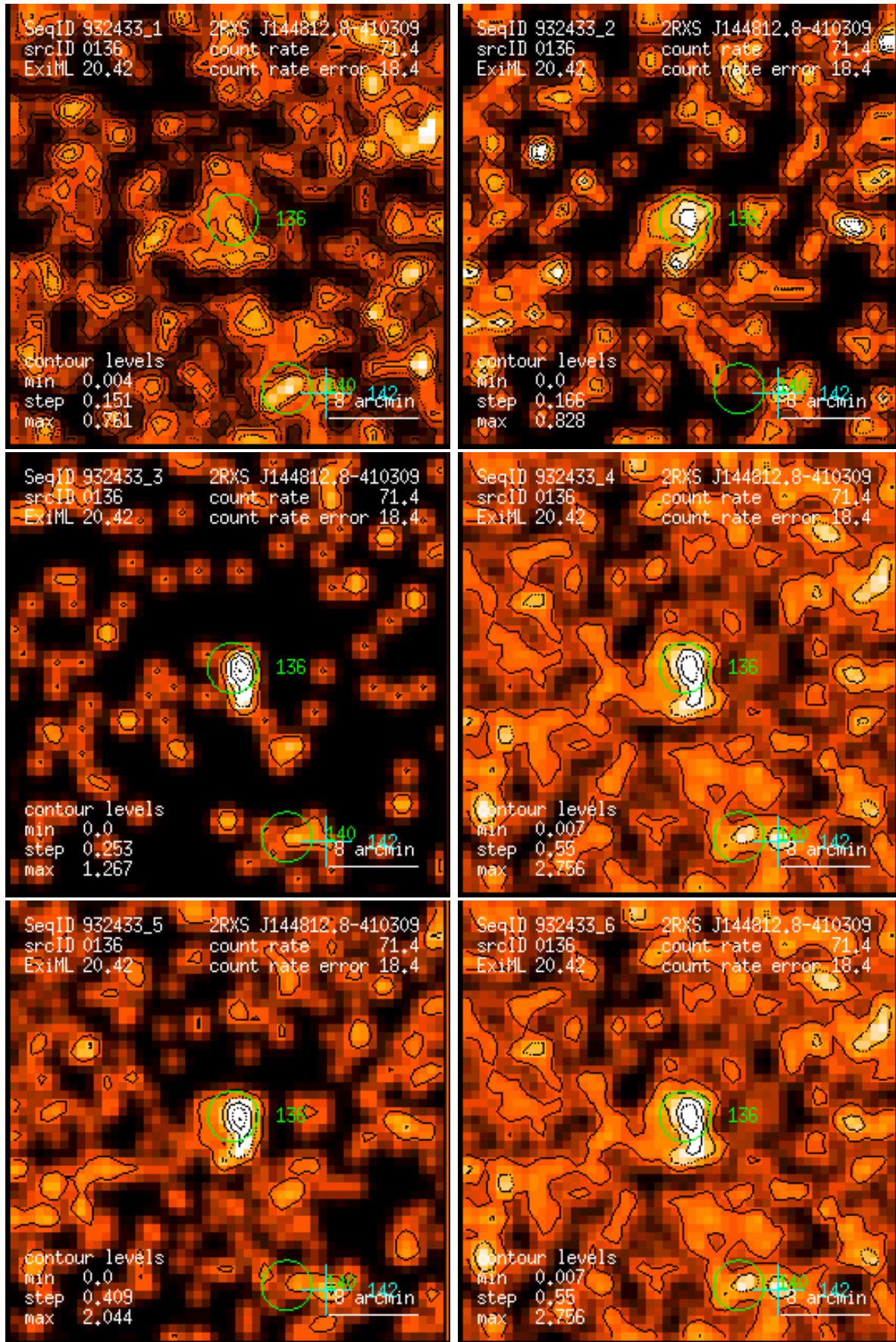
Figure 136: RASS 932433: detection 0136: band rate images, Gaussian filter: (1) PSPC channels 11 – 41, (2) 52 – 90, (3) 91 – 201, (4) 11 – 235, (5) 52 – 201, (6) 11 – 201. Broad band rates in counts/ks. Band rate contour levels in counts/ks/arcmin 2 .
