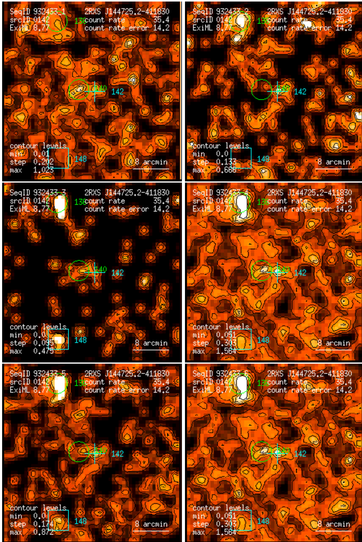
Figure 142: RASS 932433: detection 0142: band rate images, Gaussian filter: (1) PSPC channels 11 – 41, (2) 52 – 90, (3) 91 – 201, (4) 11 – 235, (5) 52 – 201, (6) 11 – 201. Broad band rates in counts/ks. Band rate contour levels in counts/ks/arcmin 2 .
