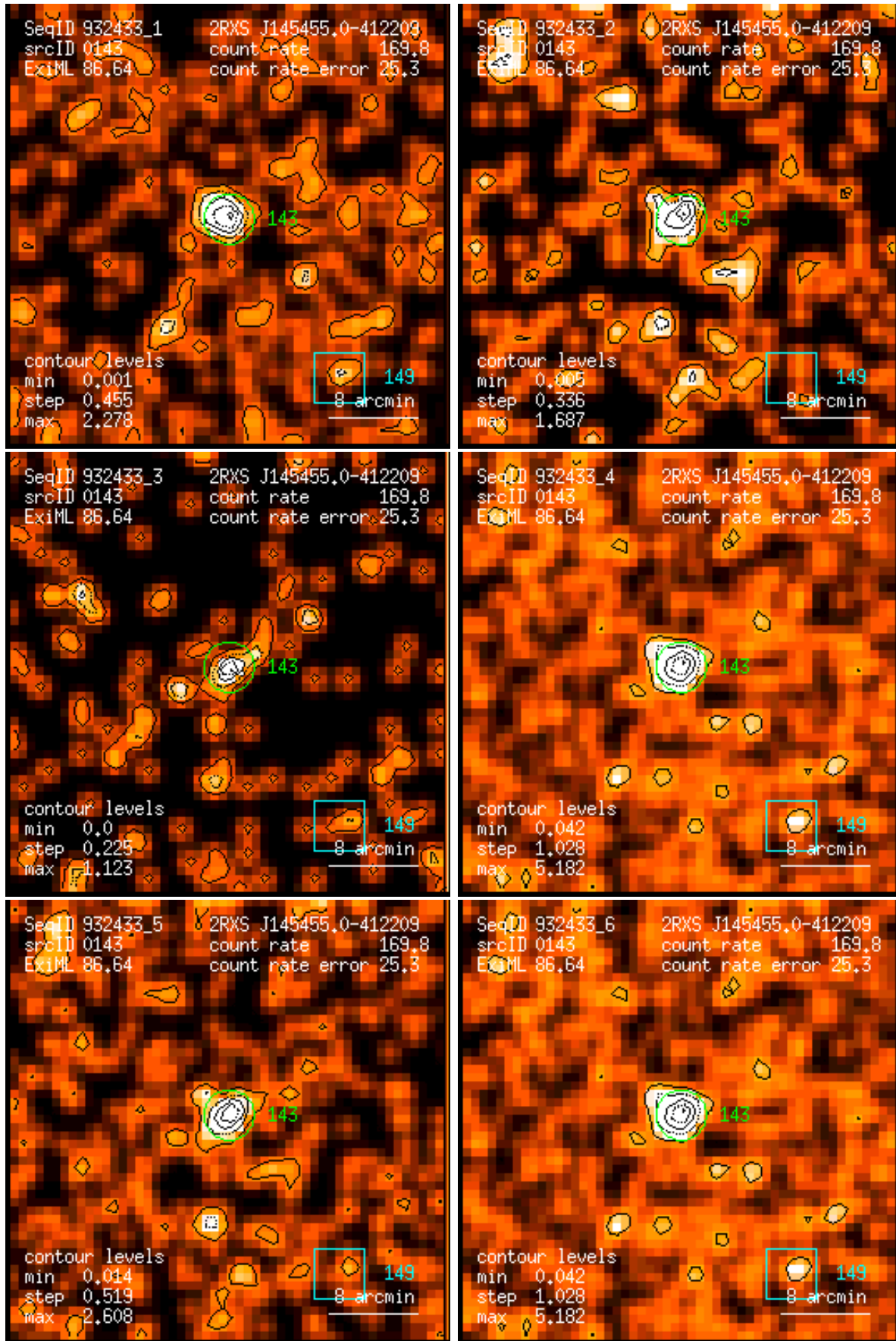
Figure 143: RASS 932433: detection 0143: band rate images, Gaussian filter: (1) PSPC channels 11 – 41, (2) 52 – 90, (3) 91 – 201, (4) 11 – 235, (5) 52 – 201, (6) 11 – 201. Broad band rates in counts/ks. Band rate contour levels in counts/ks/arcmin 2 .
