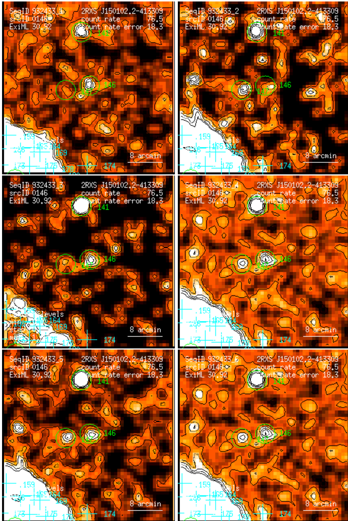
Figure 146: RASS 932433: detection 0146: band rate images, Gaussian filter: (1) PSPC channels 11 – 41, (2) 52 – 90, (3) 91 – 201, (4) 11 – 235, (5) 52 – 201, (6) 11 – 201. Broad band rates in counts/ks. Band rate contour levels in counts/ks/arcmin 2 .
