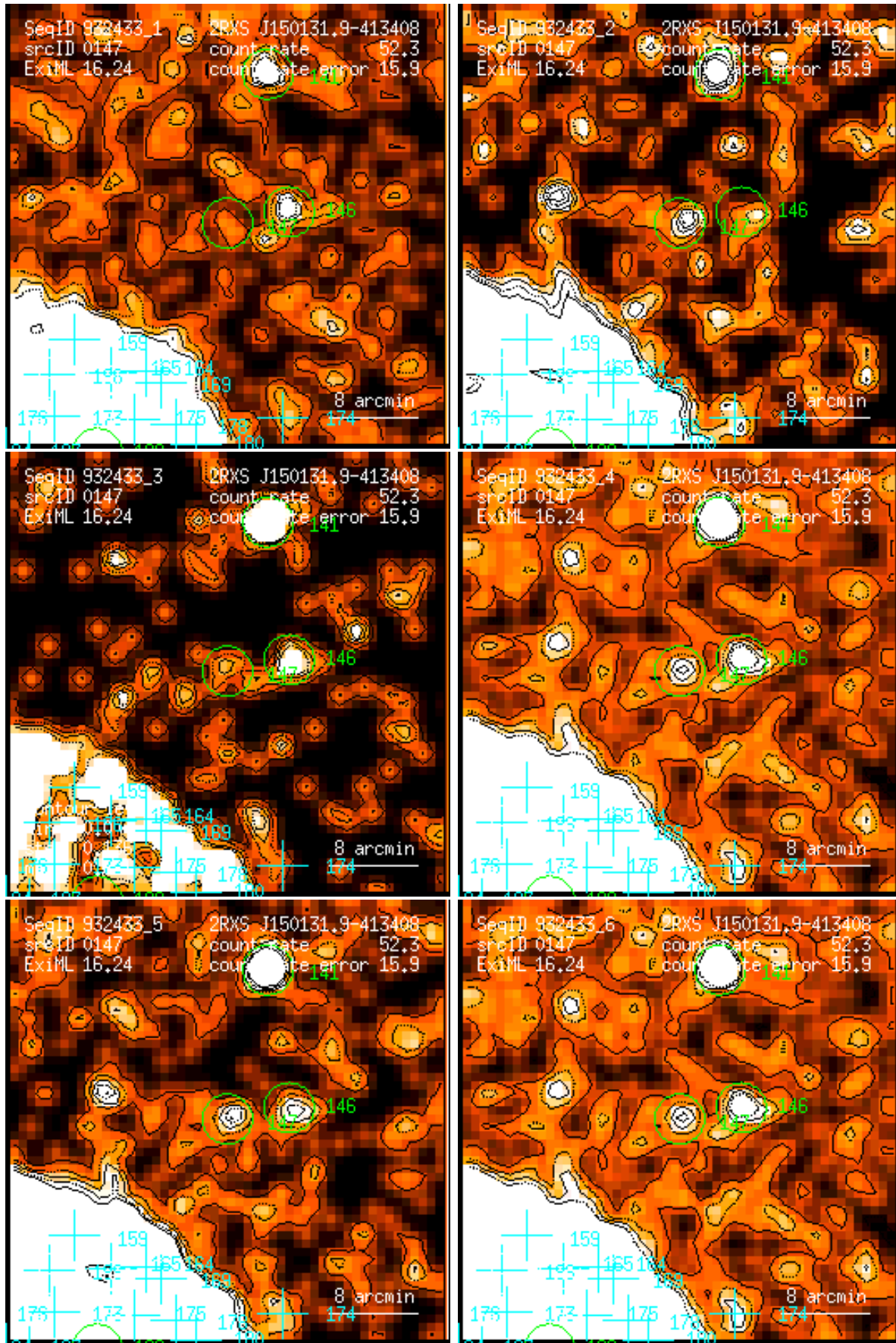
Figure 147: RASS 932433: detection 0147: band rate images, Gaussian filter: (1) PSPC channels 11 – 41, (2) 52 – 90, (3) 91 – 201, (4) 11 – 235, (5) 52 – 201, (6) 11 – 201. Broad band rates in counts/ks. Band rate contour levels in counts/ks/arcmin 2 .
