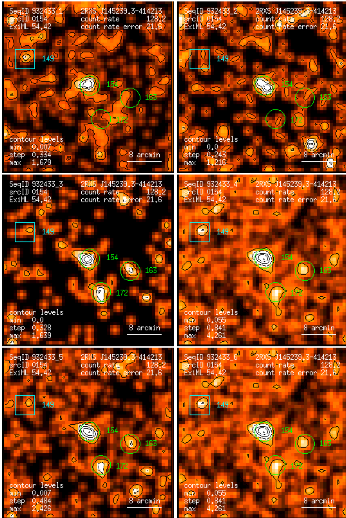
Figure 154: RASS 932433: detection 0154: band rate images, Gaussian filter: (1) PSPC channels 11 – 41, (2) 52 – 90, (3) 91 – 201, (4) 11 – 235, (5) 52 – 201, (6) 11 – 201. Broad band rates in counts/ks. Band rate contour levels in counts/ks/arcmin 2 .
