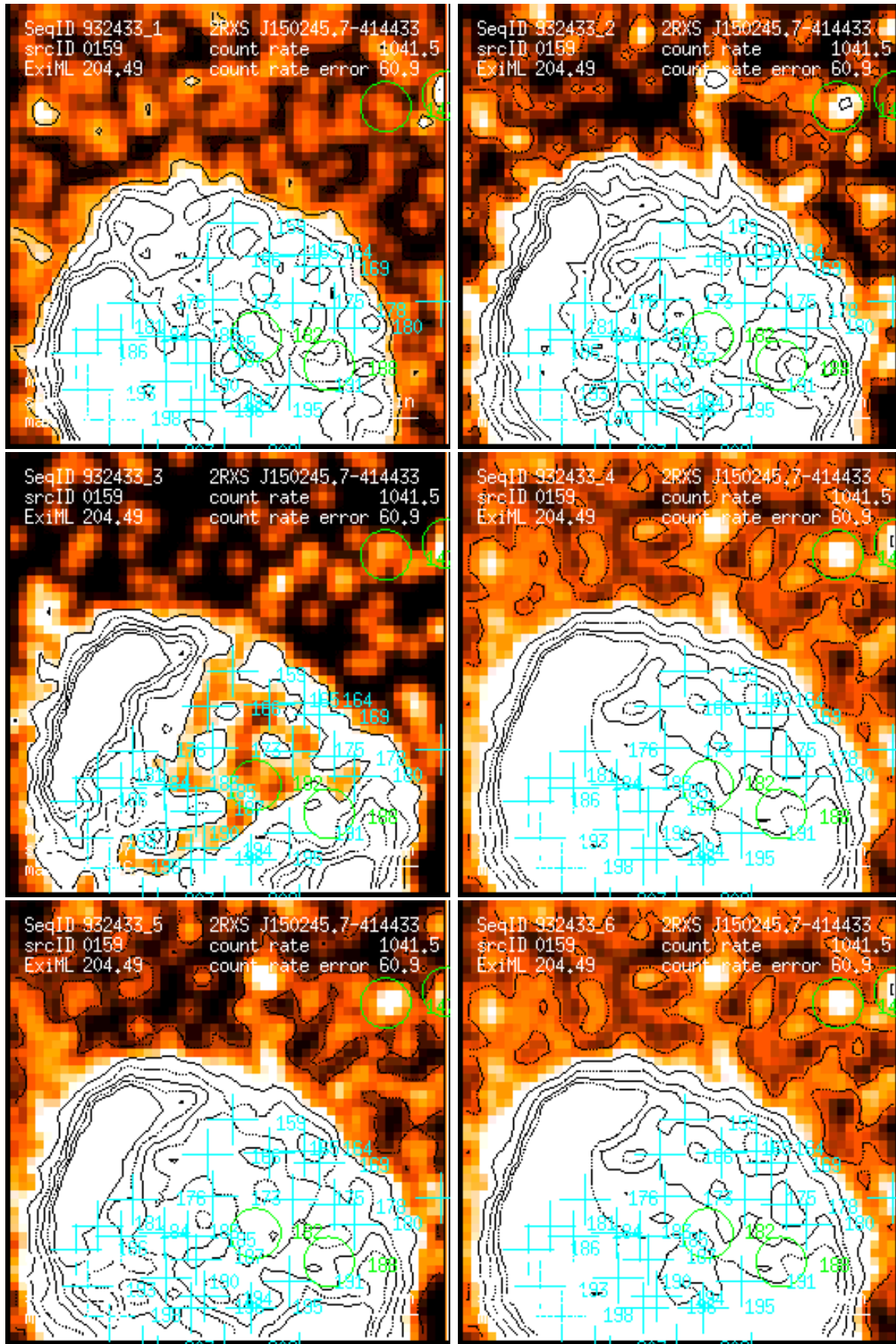
Figure 159: RASS 932433: detection 0159: band rate images, Gaussian filter: (1) PSPC channels 11 – 41, (2) 52 – 90, (3) 91 – 201, (4) 11 – 235, (5) 52 – 201, (6) 11 – 201. Broad band rates in counts/ks. Band rate contour levels in counts/ks/arcmin 2 .
