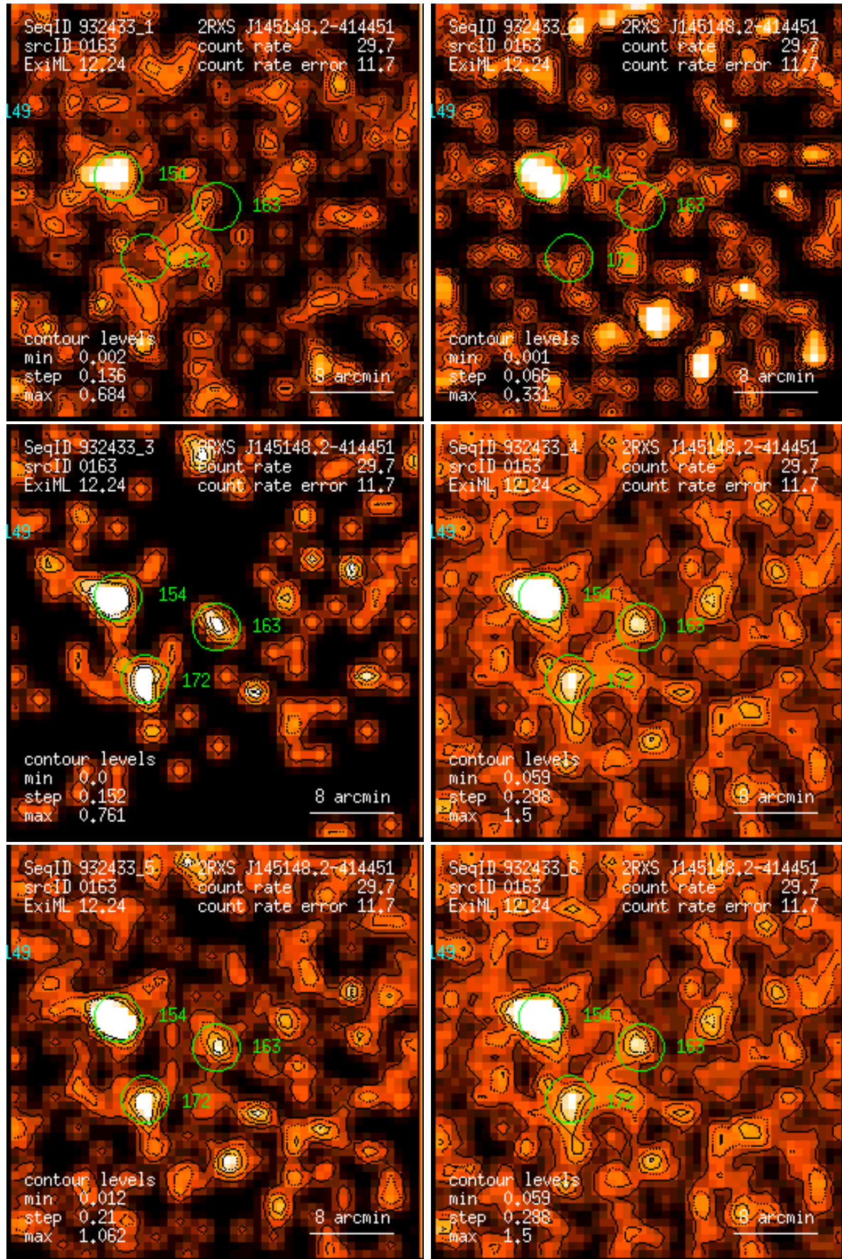
Figure 163: RASS 932433: detection 0163: band rate images, Gaussian filter: (1) PSPC channels 11 – 41, (2) 52 – 90, (3) 91 – 201, (4) 11 – 235, (5) 52 – 201, (6) 11 – 201. Broad band rates in counts/ks. Band rate contour levels in counts/ks/arcmin 2 .
