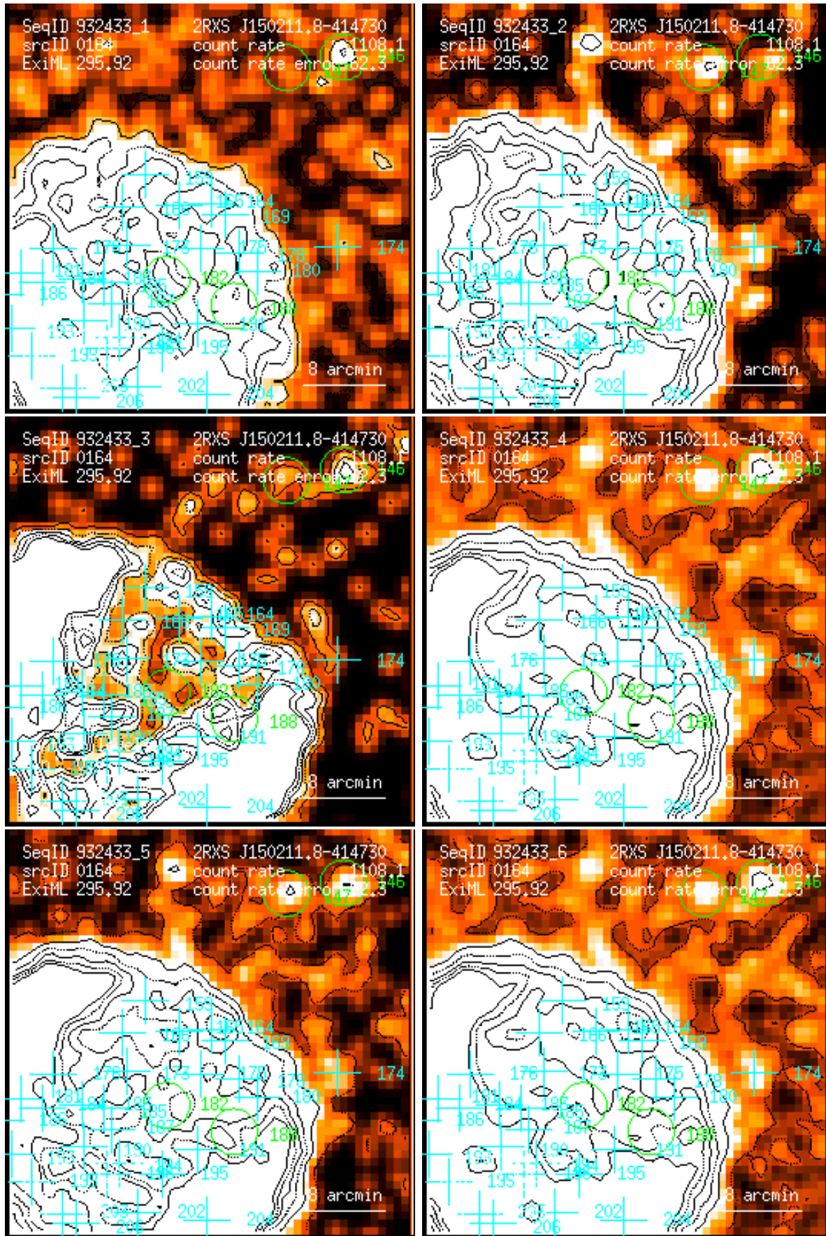
Figure 164: RASS 932433: detection 0164: band rate images, Gaussian filter: (1) PSPC channels 11 – 41, (2) 52 – 90, (3) 91 – 201, (4) 11 – 235, (5) 52 – 201, (6) 11 – 201. Broad band rates in counts/ks. Band rate contour levels in counts/ks/arcmin 2 .
