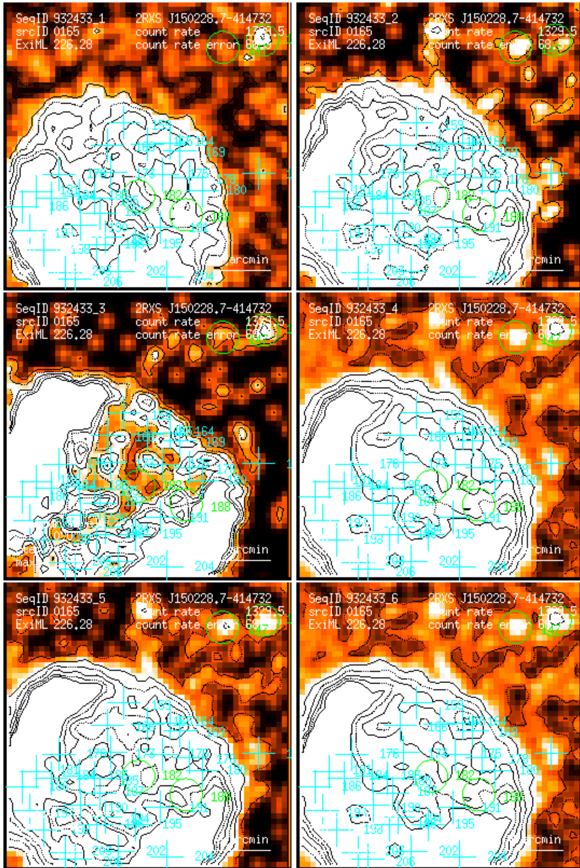
Figure 165: RASS 932433: detection 0165: band rate images, Gaussian filter: (1) PSPC channels 11 – 41, (2) 52 – 90, (3) 91 – 201, (4) 11 – 235, (5) 52 – 201, (6) 11 – 201. Broad band rates in counts/ks. Band rate contour levels in counts/ks/arcmin 2 .
