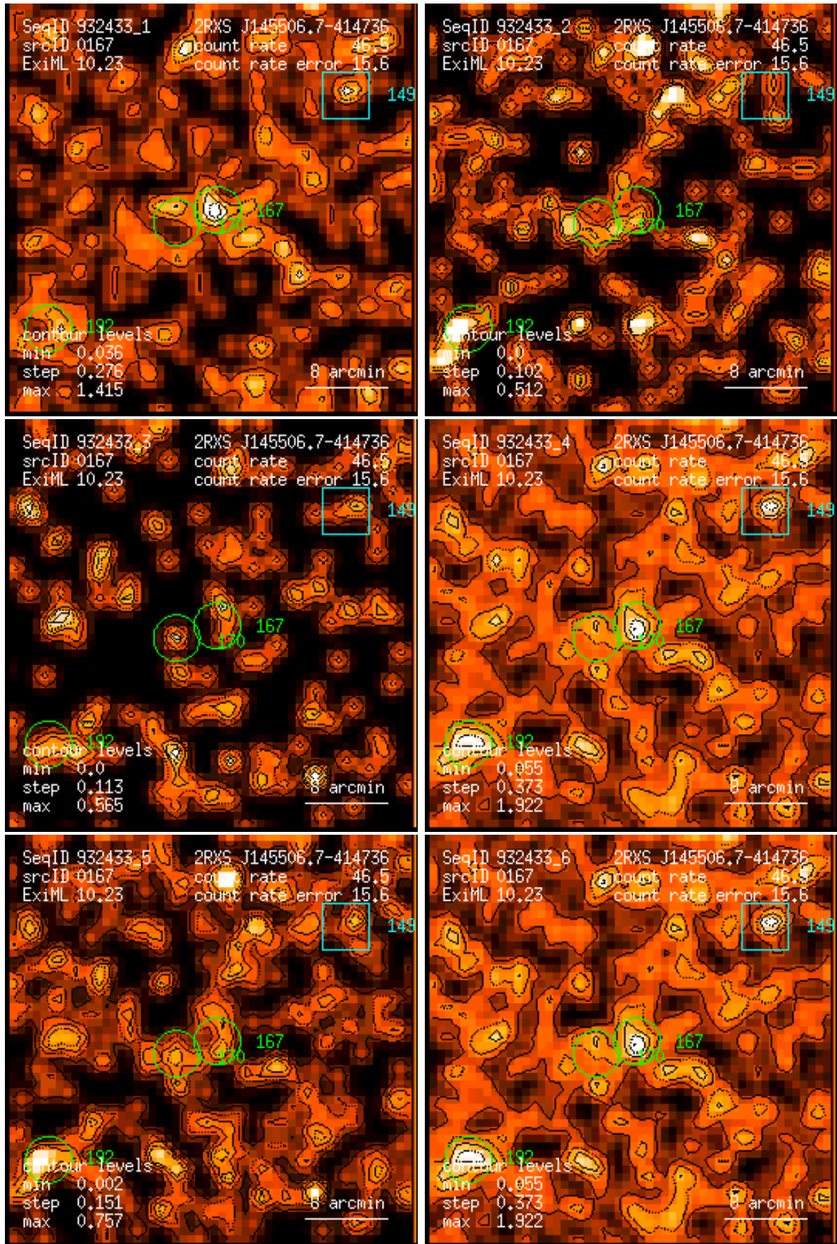
Figure 167: RASS 932433: detection 0167: band rate images, Gaussian filter: (1) PSPC channels 11 – 41, (2) 52 – 90, (3) 91 – 201, (4) 11 – 235, (5) 52 – 201, (6) 11 – 201. Broad band rates in counts/ks. Band rate contour levels in counts/ks/arcmin 2 .
