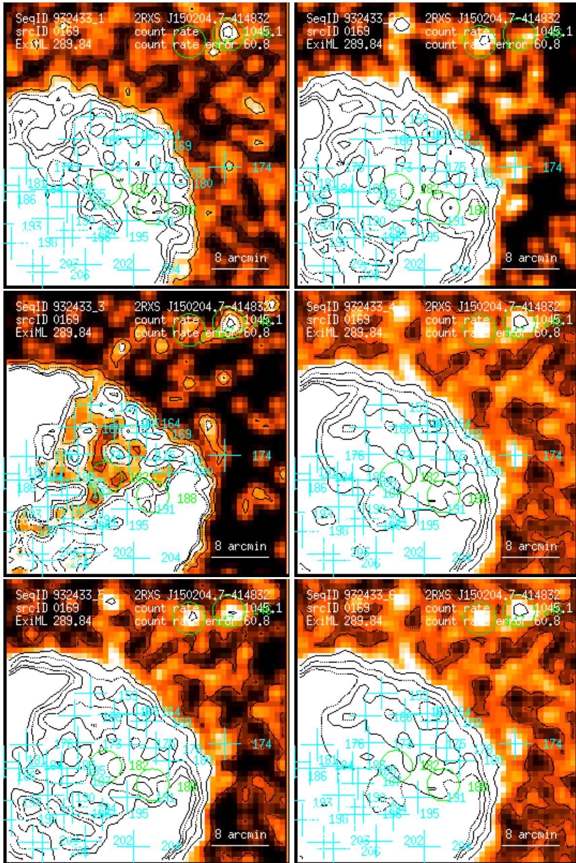
Figure 169: RASS 932433: detection 0169: band rate images, Gaussian filter: (1) PSPC channels 11 – 41, (2) 52 – 90, (3) 91 – 201, (4) 11 – 235, (5) 52 – 201, (6) 11 – 201. Broad band rates in counts/ks. Band rate contour levels in counts/ks/arcmin 2 .
