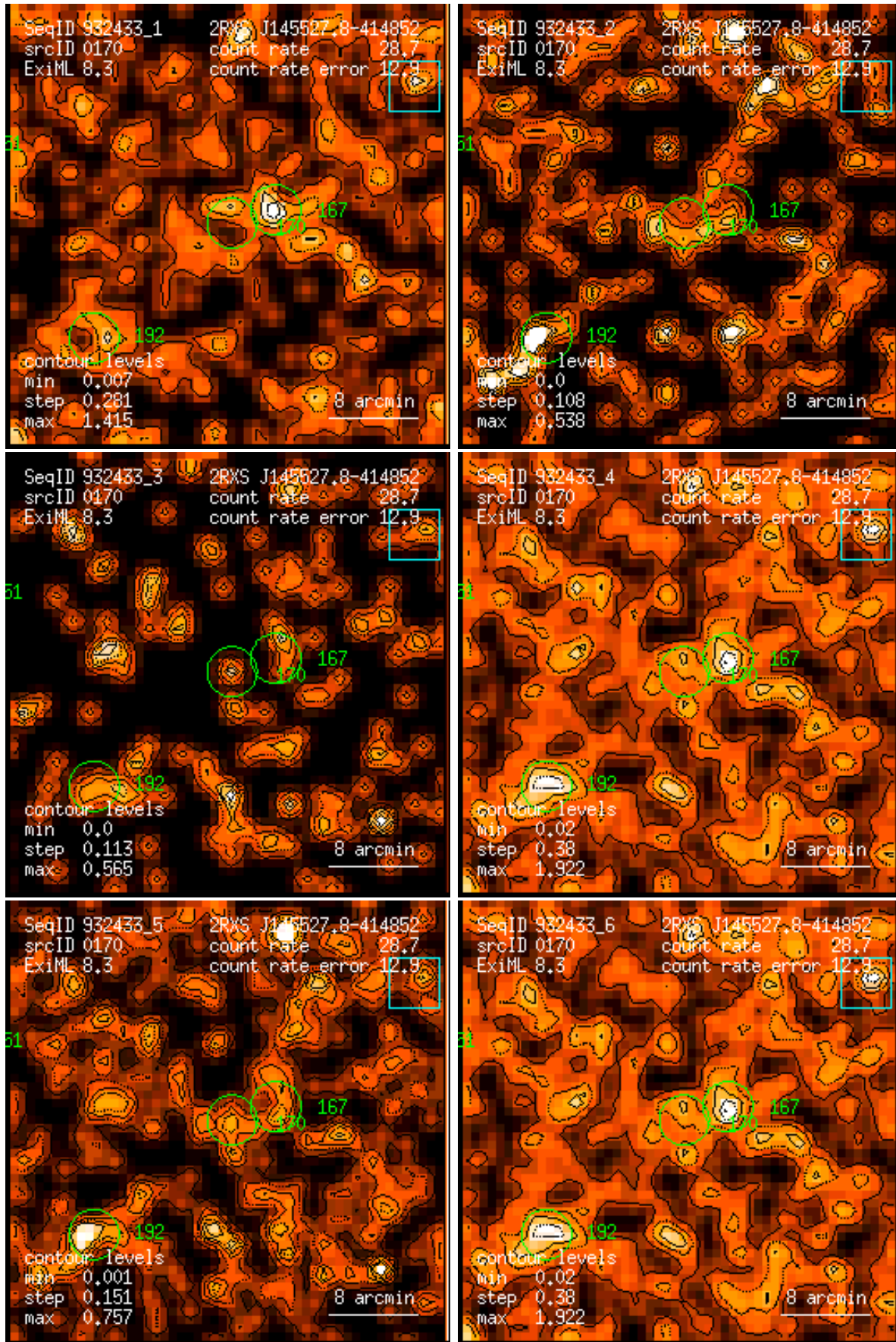
Figure 170: RASS 932433: detection 0170: band rate images, Gaussian filter: (1) PSPC channels 11 – 41, (2) 52 – 90, (3) 91 – 201, (4) 11 – 235, (5) 52 – 201, (6) 11 – 201. Broad band rates in counts/ks. Band rate contour levels in counts/ks/arcmin 2 .
