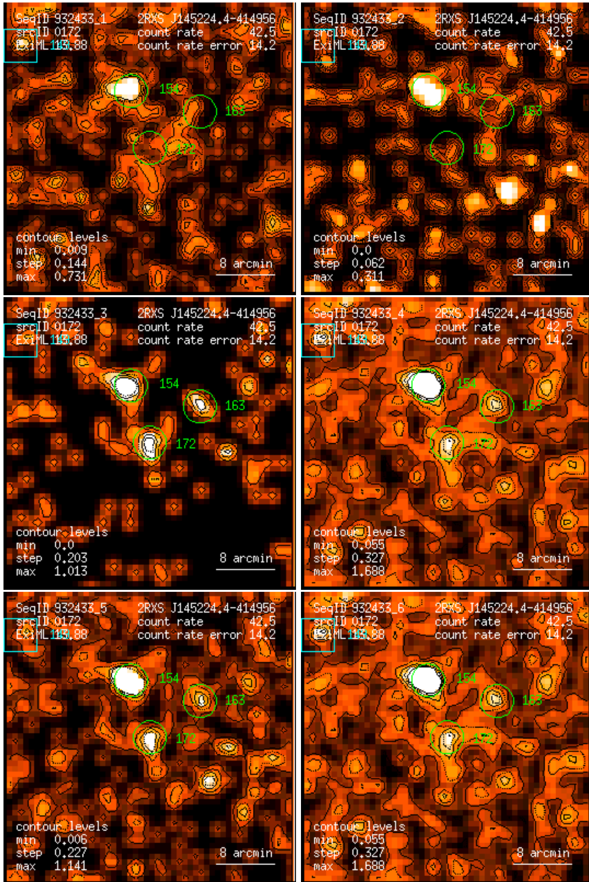
Figure 172: RASS 932433: detection 0172: band rate images, Gaussian filter: (1) PSPC channels 11 – 41, (2) 52 – 90, (3) 91 – 201, (4) 11 – 235, (5) 52 – 201, (6) 11 – 201. Broad band rates in counts/ks. Band rate contour levels in counts/ks/arcmin 2 .
