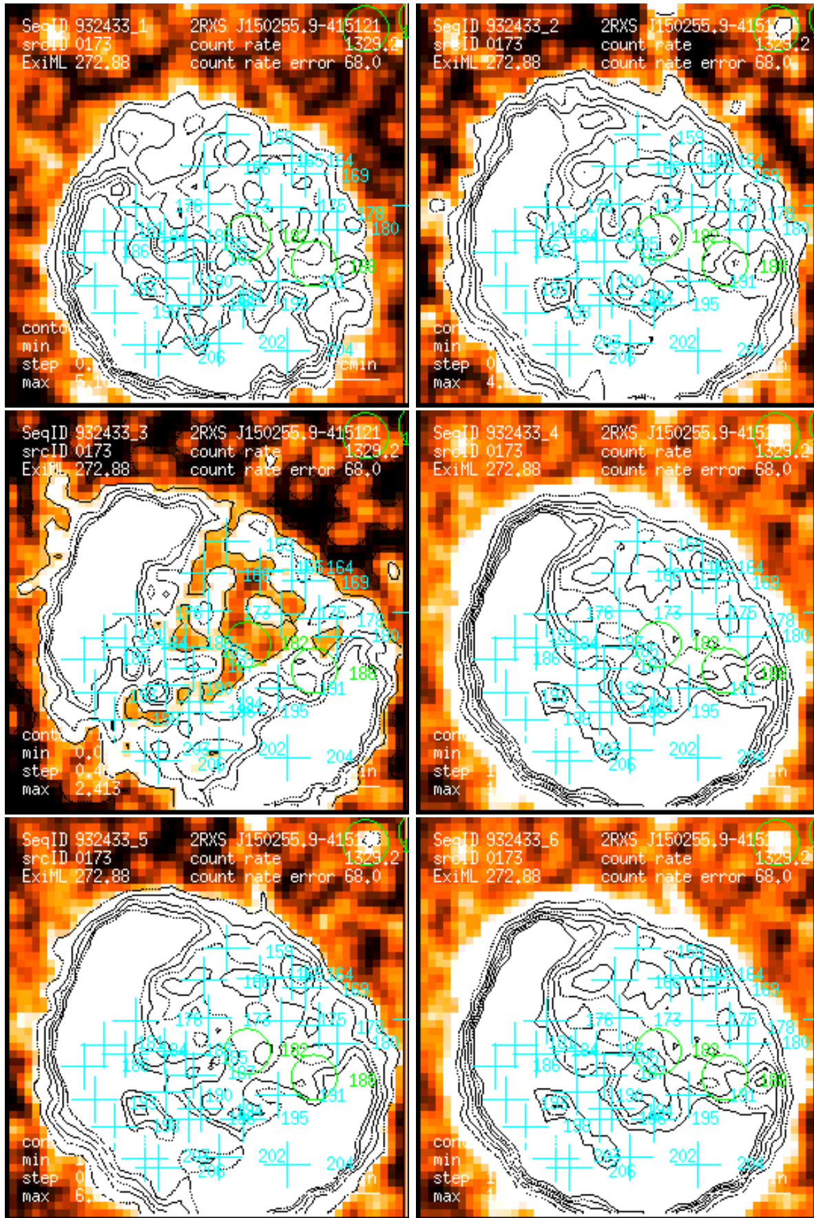
Figure 173: RASS 932433: detection 0173: band rate images, Gaussian filter: (1) PSPC channels 11 – 41, (2) 52 – 90, (3) 91 – 201, (4) 11 – 235, (5) 52 – 201, (6) 11 – 201. Broad band rates in counts/ks. Band rate contour levels in counts/ks/arcmin 2 .
