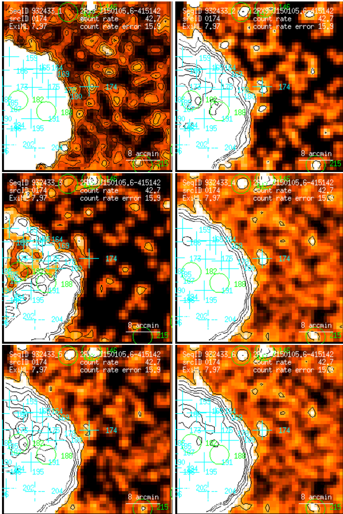
Figure 174: RASS 932433: detection 0174: band rate images, Gaussian filter: (1) PSPC channels 11 – 41, (2) 52 – 90, (3) 91 – 201, (4) 11 – 235, (5) 52 – 201, (6) 11 – 201. Broad band rates in counts/ks. Band rate contour levels in counts/ks/arcmin 2 .
