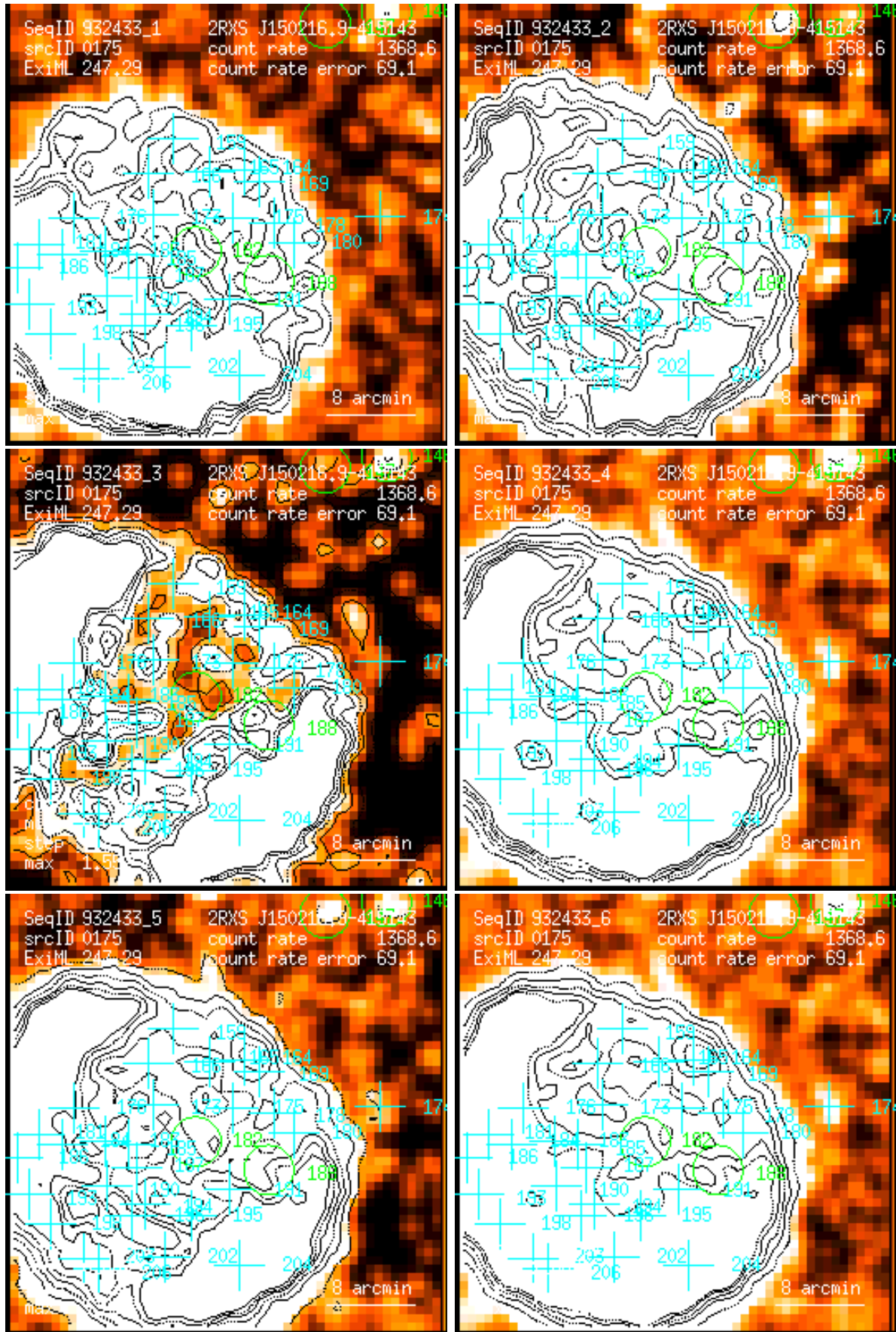
Figure 175: RASS 932433: detection 0175: band rate images, Gaussian filter: (1) PSPC channels 11 – 41, (2) 52 – 90, (3) 91 – 201, (4) 11 – 235, (5) 52 – 201, (6) 11 – 201. Broad band rates in counts/ks. Band rate contour levels in counts/ks/arcmin 2 .
