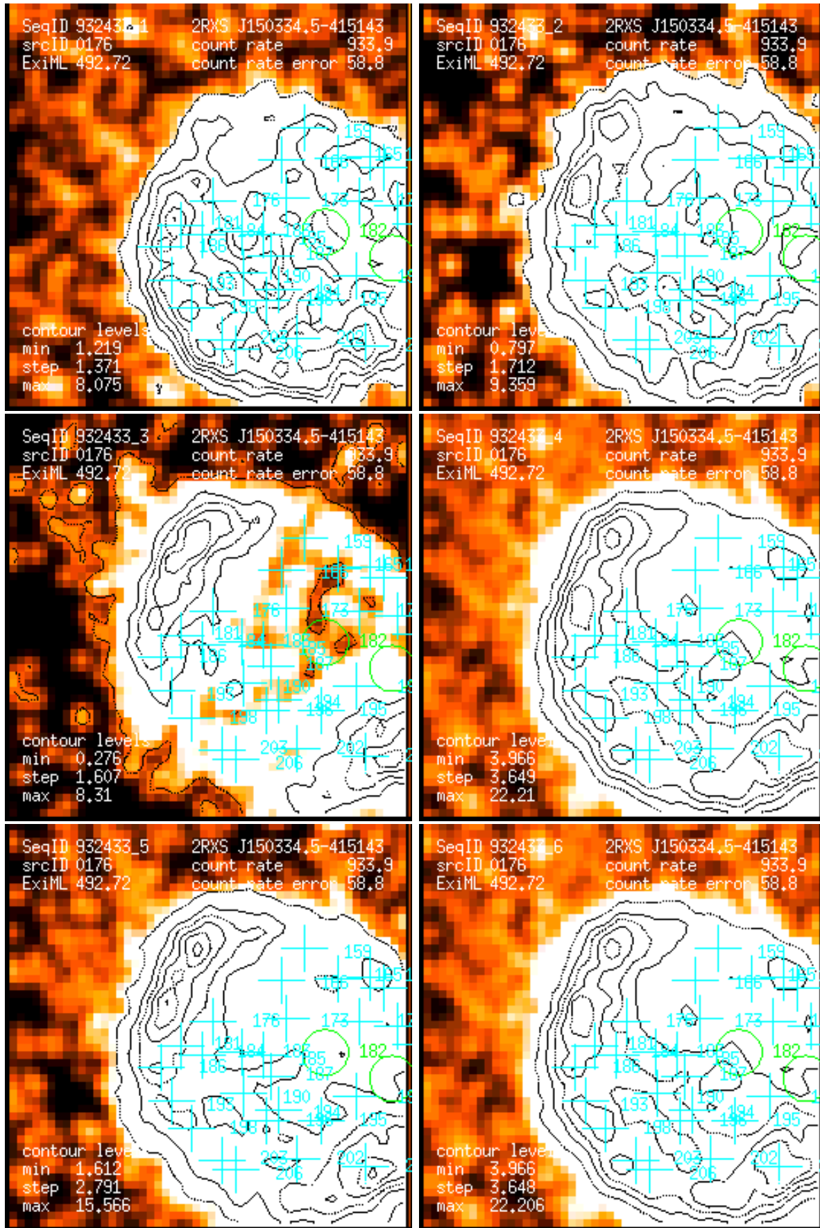
Figure 176: RASS 932433: detection 0176: band rate images, Gaussian filter: (1) PSPC channels 11 – 41, (2) 52 – 90, (3) 91 – 201, (4) 11 – 235, (5) 52 – 201, (6) 11 – 201. Broad band rates in counts/ks. Band rate contour levels in counts/ks/arcmin 2 .
