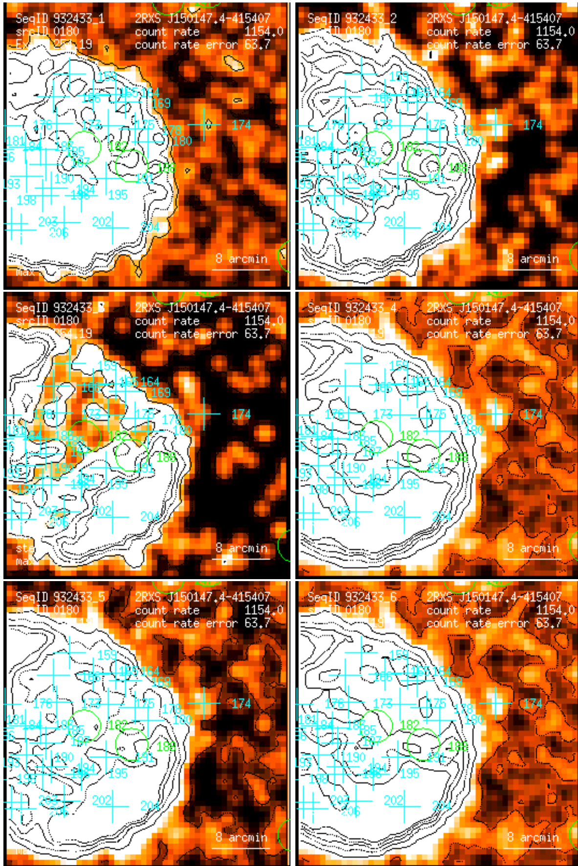
Figure 180: RASS 932433: detection 0180: band rate images, Gaussian filter: (1) PSPC channels 11 – 41, (2) 52 – 90, (3) 91 – 201, (4) 11 – 235, (5) 52 – 201, (6) 11 – 201. Broad band rates in counts/ks. Band rate contour levels in counts/ks/arcmin 2 .
