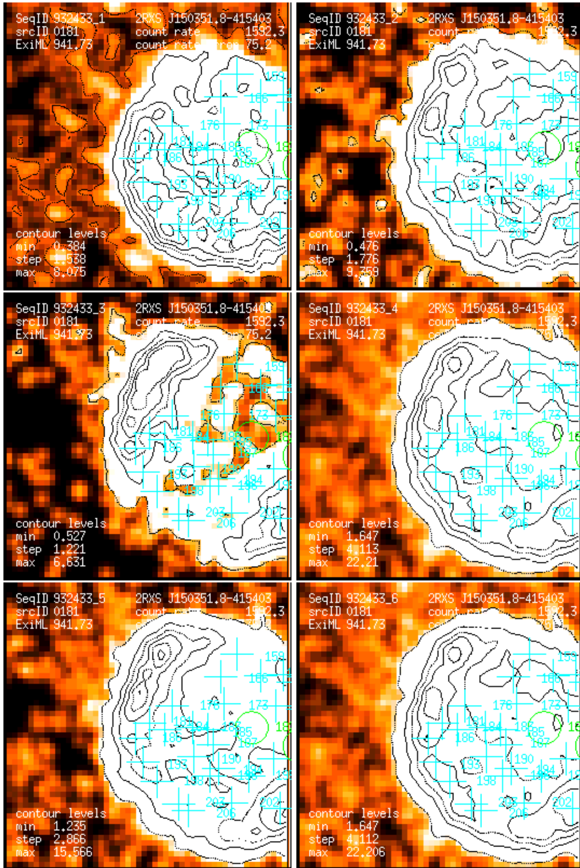
Figure 181: RASS 932433: detection 0181: band rate images, Gaussian filter: (1) PSPC channels 11 – 41, (2) 52 – 90, (3) 91 – 201, (4) 11 – 235, (5) 52 – 201, (6) 11 – 201. Broad band rates in counts/ks. Band rate contour levels in counts/ks/arcmin 2 .
