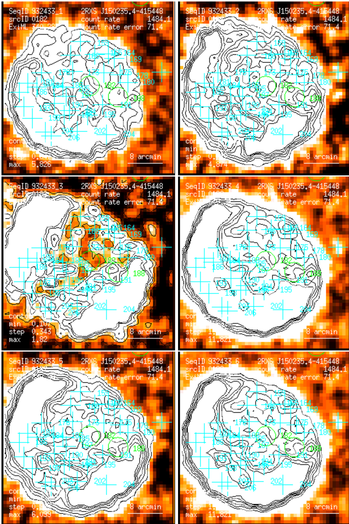
Figure 182: RASS 932433: detection 0182: band rate images, Gaussian filter: (1) PSPC channels 11 – 41, (2) 52 – 90, (3) 91 – 201, (4) 11 – 235, (5) 52 – 201, (6) 11 – 201. Broad band rates in counts/ks. Band rate contour levels in counts/ks/arcmin 2 .
