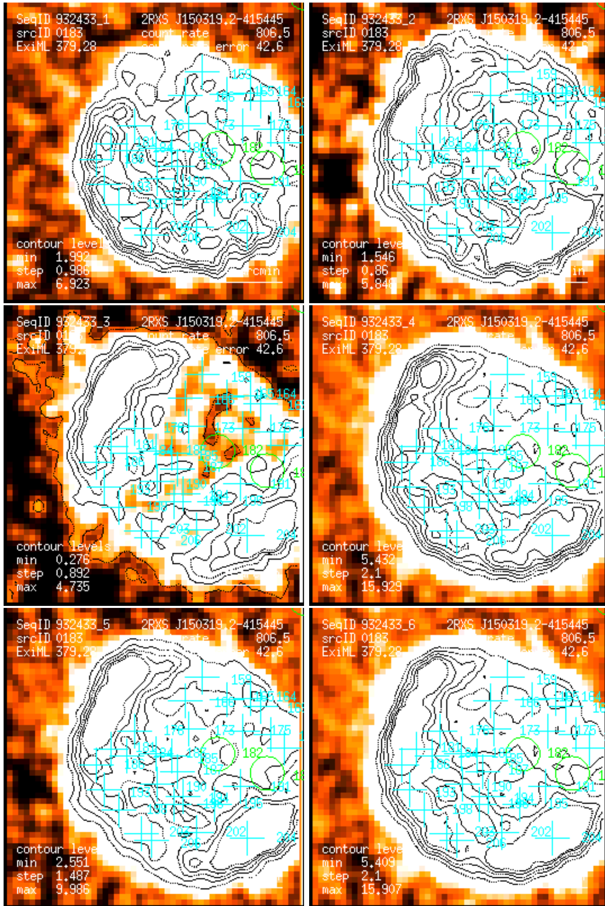
Figure 183: RASS 932433: detection 0183: band rate images, Gaussian filter: (1) PSPC channels 11 – 41, (2) 52 – 90, (3) 91 – 201, (4) 11 – 235, (5) 52 – 201, (6) 11 – 201. Broad band rates in counts/ks. Band rate contour levels in counts/ks/arcmin 2 .
