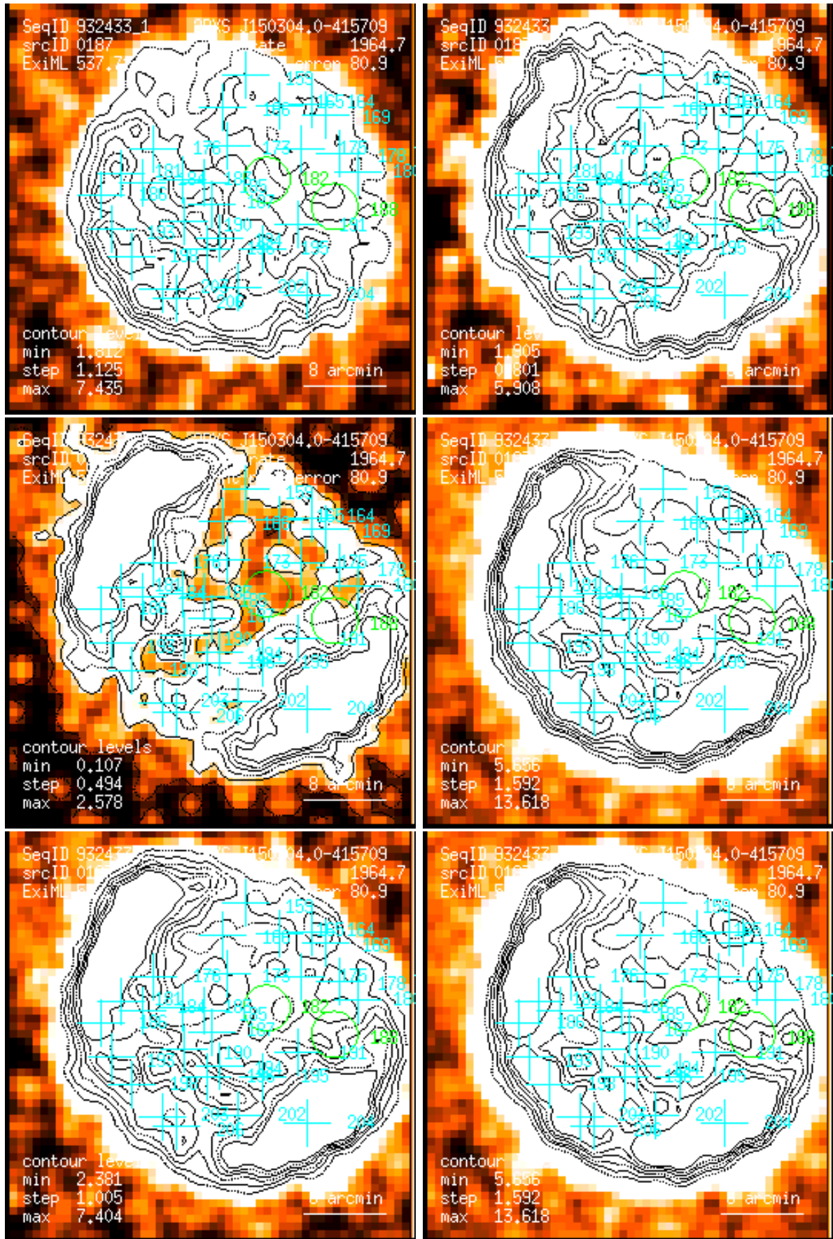
Figure 187: RASS 932433: detection 0187: band rate images, Gaussian filter: (1) PSPC channels 11 – 41, (2) 52 – 90, (3) 91 – 201, (4) 11 – 235, (5) 52 – 201, (6) 11 – 201. Broad band rates in counts/ks. Band rate contour levels in counts/ks/arcmin 2 .
