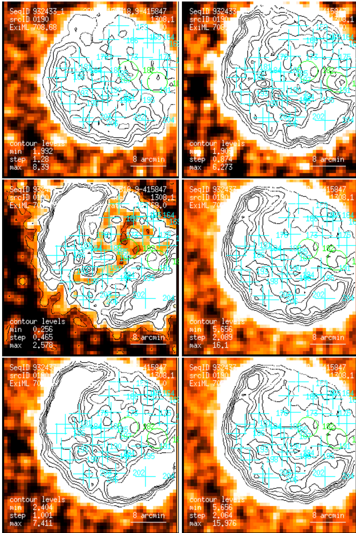
Figure 190: RASS 932433: detection 0190: band rate images, Gaussian filter: (1) PSPC channels 11 – 41, (2) 52 – 90, (3) 91 – 201, (4) 11 – 235, (5) 52 – 201, (6) 11 – 201. Broad band rates in counts/ks. Band rate contour levels in counts/ks/arcmin 2 .
