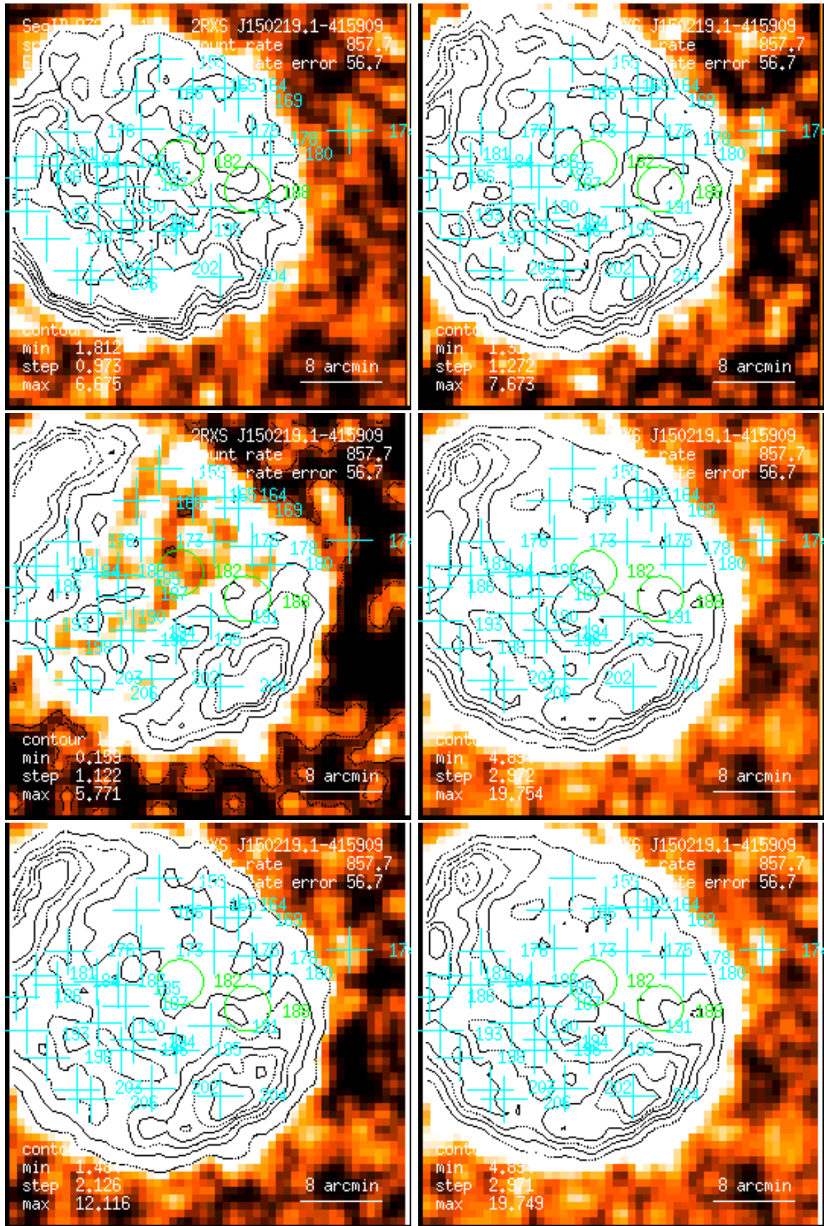
Figure 191: RASS 932433: detection 0191: band rate images, Gaussian filter: (1) PSPC channels 11 – 41, (2) 52 – 90, (3) 91 – 201, (4) 11 – 235, (5) 52 – 201, (6) 11 – 201. Broad band rates in counts/ks. Band rate contour levels in counts/ks/arcmin 2 .
