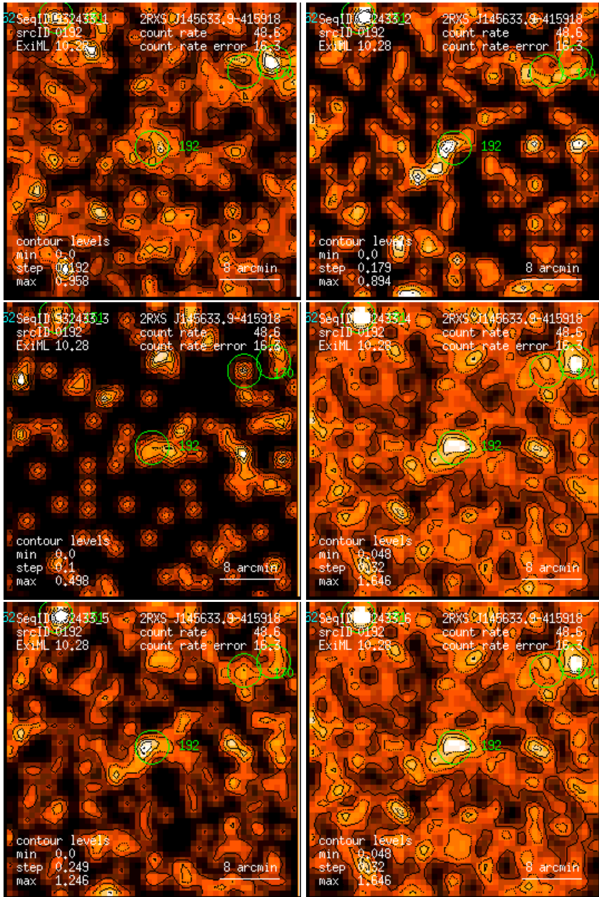
Figure 192: RASS 932433: detection 0192: band rate images, Gaussian filter: (1) PSPC channels 11 – 41, (2) 52 – 90, (3) 91 – 201, (4) 11 – 235, (5) 52 – 201, (6) 11 – 201. Broad band rates in counts/ks. Band rate contour levels in counts/ks/arcmin 2 .
