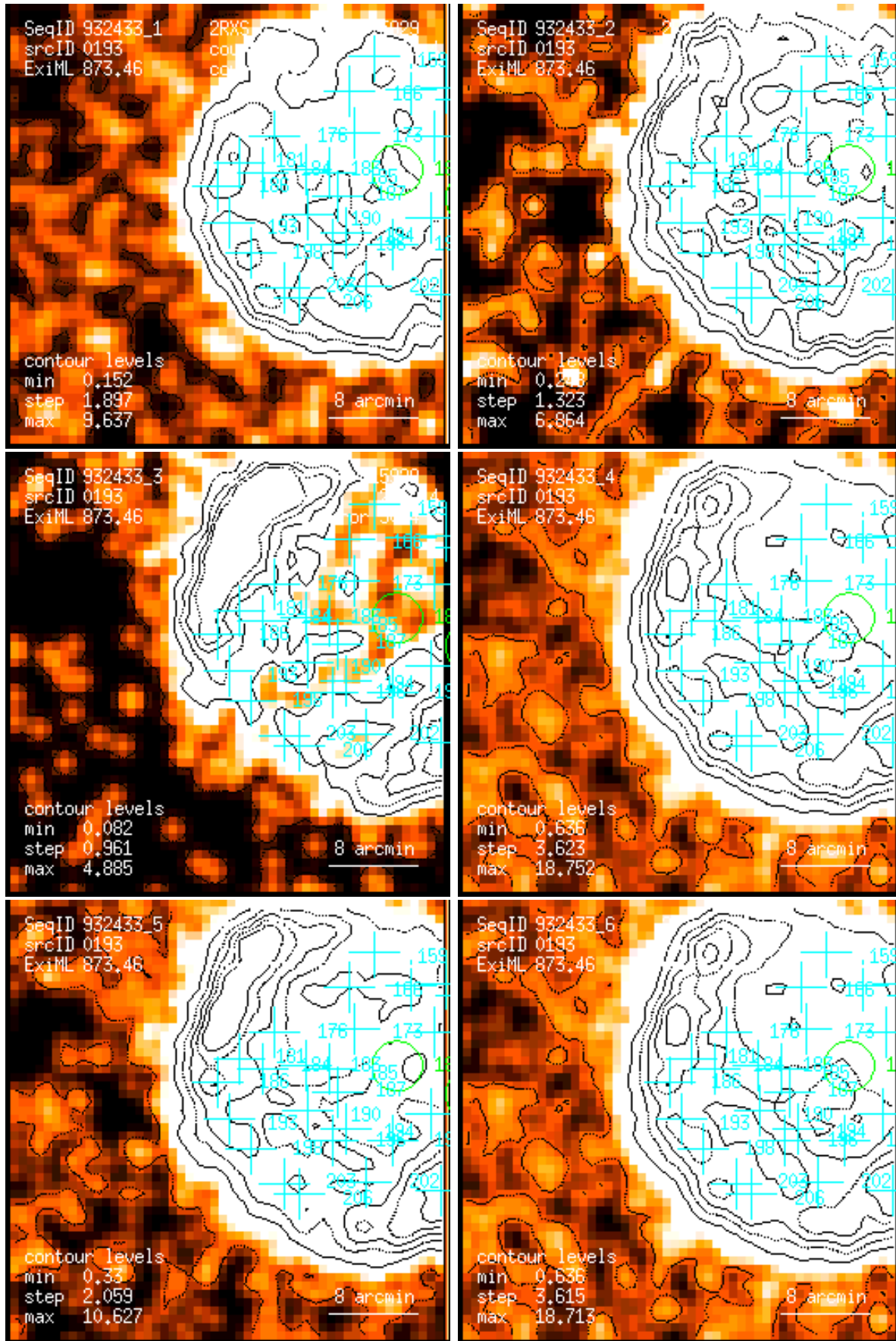
Figure 193: RASS 932433: detection 0193: band rate images, Gaussian filter: (1) PSPC channels 11 – 41, (2) 52 – 90, (3) 91 – 201, (4) 11 – 235, (5) 52 – 201, (6) 11 – 201. Broad band rates in counts/ks. Band rate contour levels in counts/ks/arcmin 2 .
