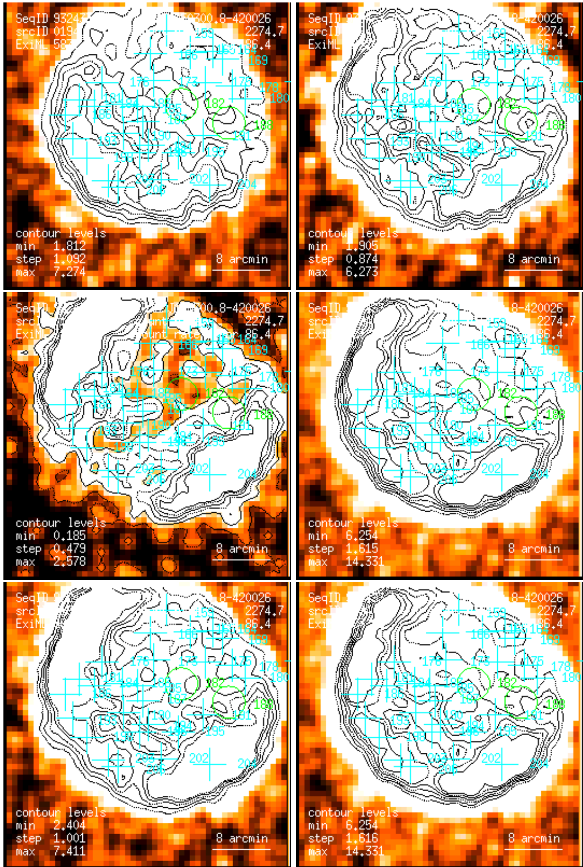
Figure 194: RASS 932433: detection 0194: band rate images, Gaussian filter: (1) PSPC channels 11 – 41, (2) 52 – 90, (3) 91 – 201, (4) 11 – 235, (5) 52 – 201, (6) 11 – 201. Broad band rates in counts/ks. Band rate contour levels in counts/ks/arcmin 2 .
