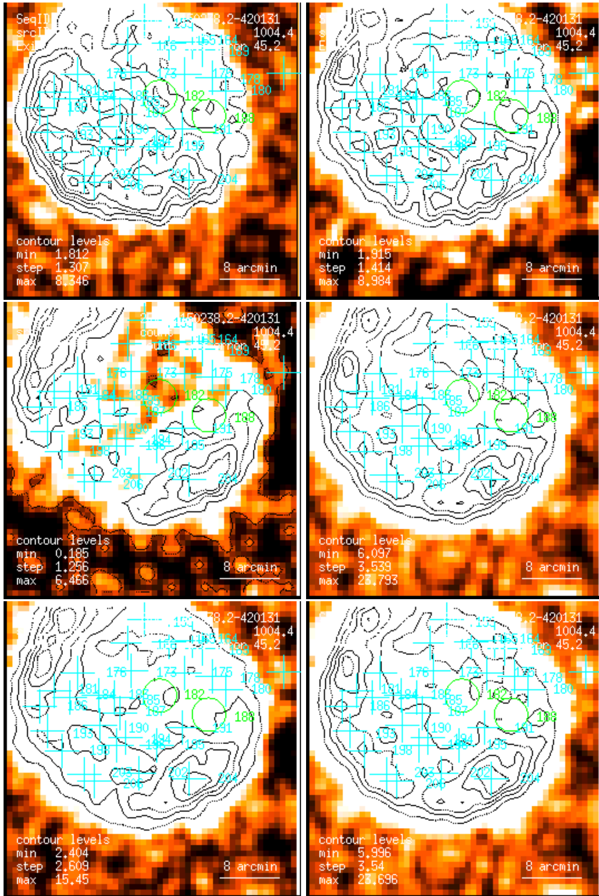
Figure 195: RASS 932433: detection 0195: band rate images, Gaussian filter: (1) PSPC channels 11 – 41, (2) 52 – 90, (3) 91 – 201, (4) 11 – 235, (5) 52 – 201, (6) 11 – 201. Broad band rates in counts/ks. Band rate contour levels in counts/ks/arcmin 2 .
