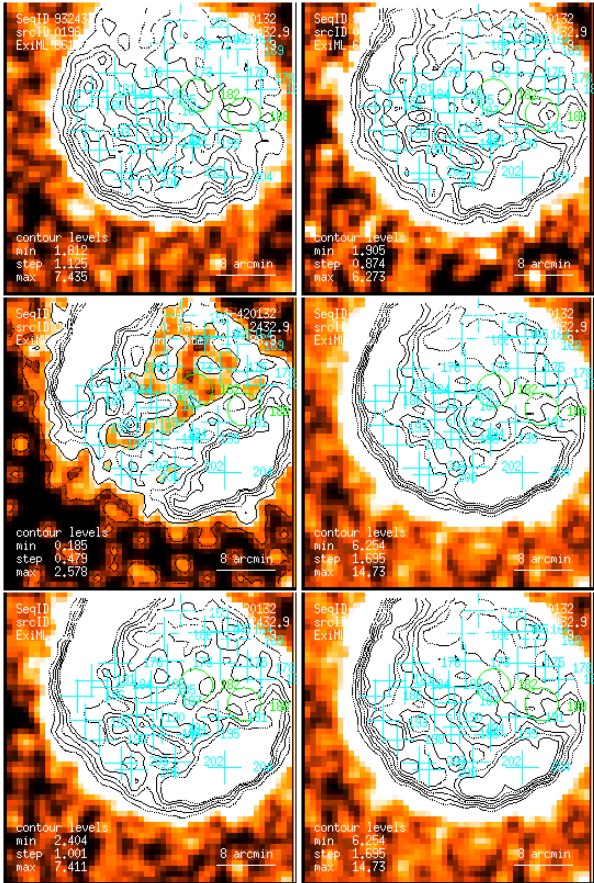
Figure 196: RASS 932433: detection 0196: band rate images, Gaussian filter: (1) PSPC channels 11 – 41, (2) 52 – 90, (3) 91 – 201, (4) 11 – 235, (5) 52 – 201, (6) 11 – 201. Broad band rates in counts/ks. Band rate contour levels in counts/ks/arcmin 2 .
