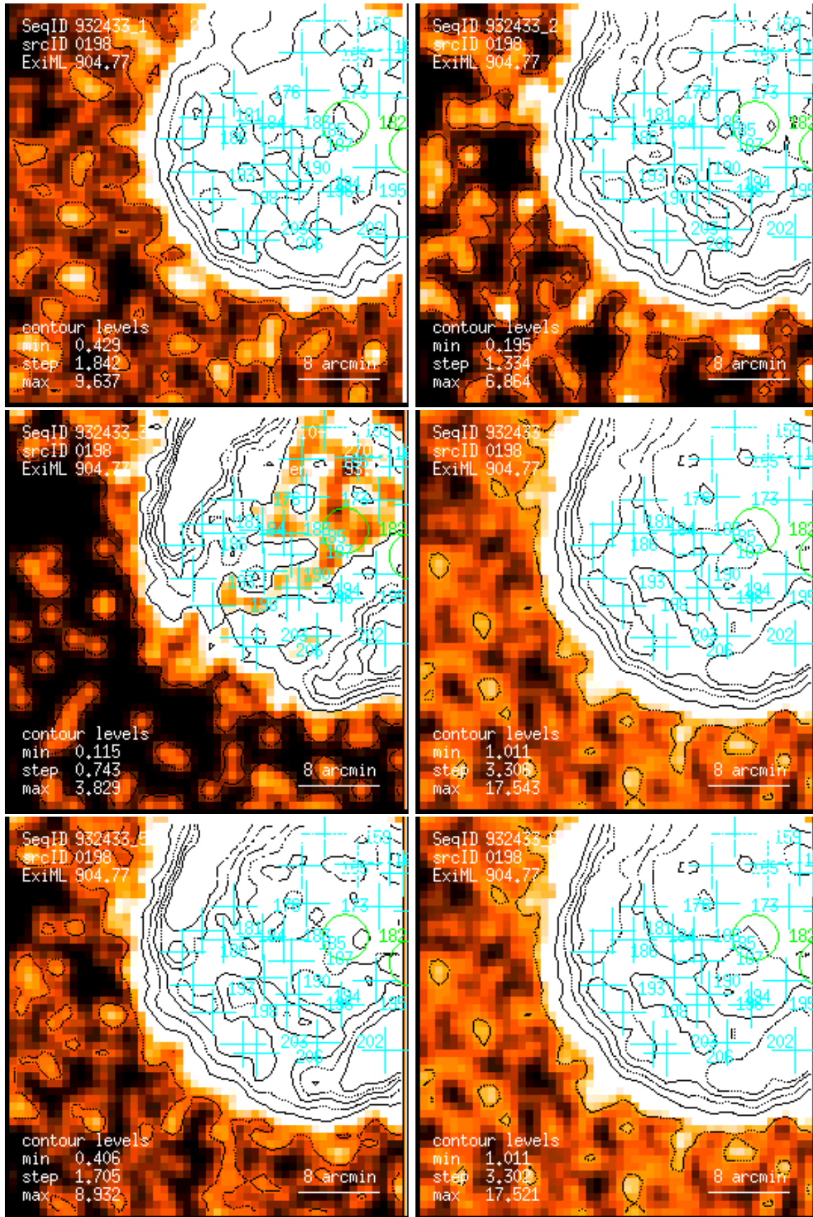
Figure 198: RASS 932433: detection 0198: band rate images, Gaussian filter: (1) PSPC channels 11 – 41, (2) 52 – 90, (3) 91 – 201, (4) 11 – 235, (5) 52 – 201, (6) 11 – 201. Broad band rates in counts/ks. Band rate contour levels in counts/ks/arcmin 2 .
