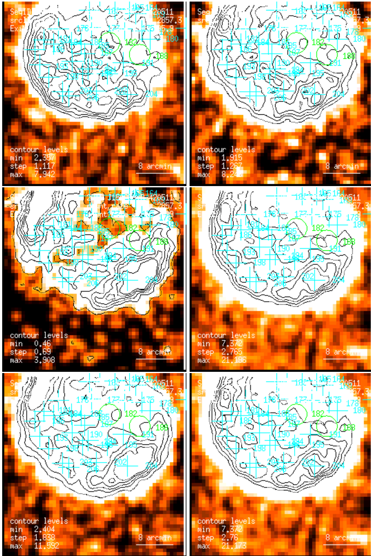
Figure 202: RASS 932433: detection 0202: band rate images, Gaussian filter: (1) PSPC channels 11 – 41, (2) 52 – 90, (3) 91 – 201, (4) 11 – 235, (5) 52 – 201, (6) 11 – 201. Broad band rates in counts/ks. Band rate contour levels in counts/ks/arcmin 2 .
