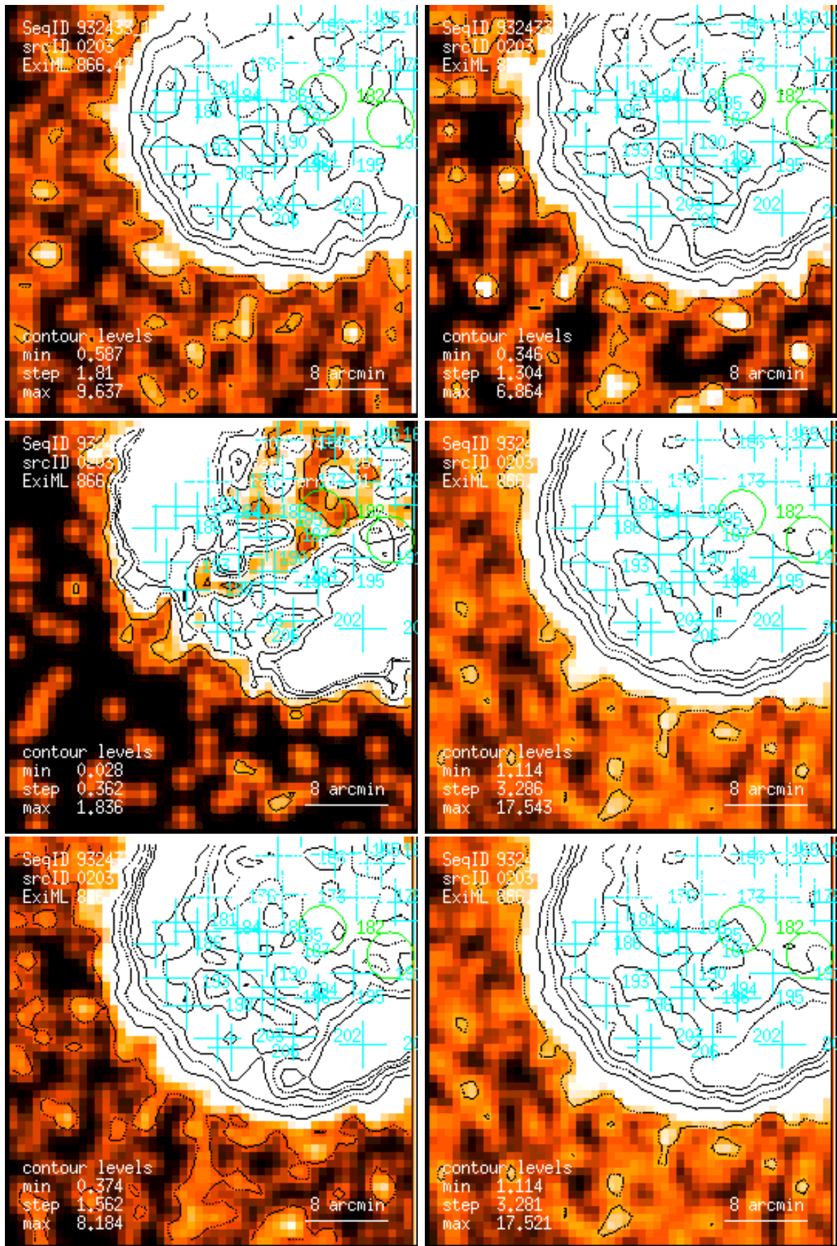
Figure 203: RASS 932433: detection 0203: band rate images, Gaussian filter: (1) PSPC channels 11 – 41, (2) 52 – 90, (3) 91 – 201, (4) 11 – 235, (5) 52 – 201, (6) 11 – 201. Broad band rates in counts/ks. Band rate contour levels in counts/ks/arcmin 2 .
