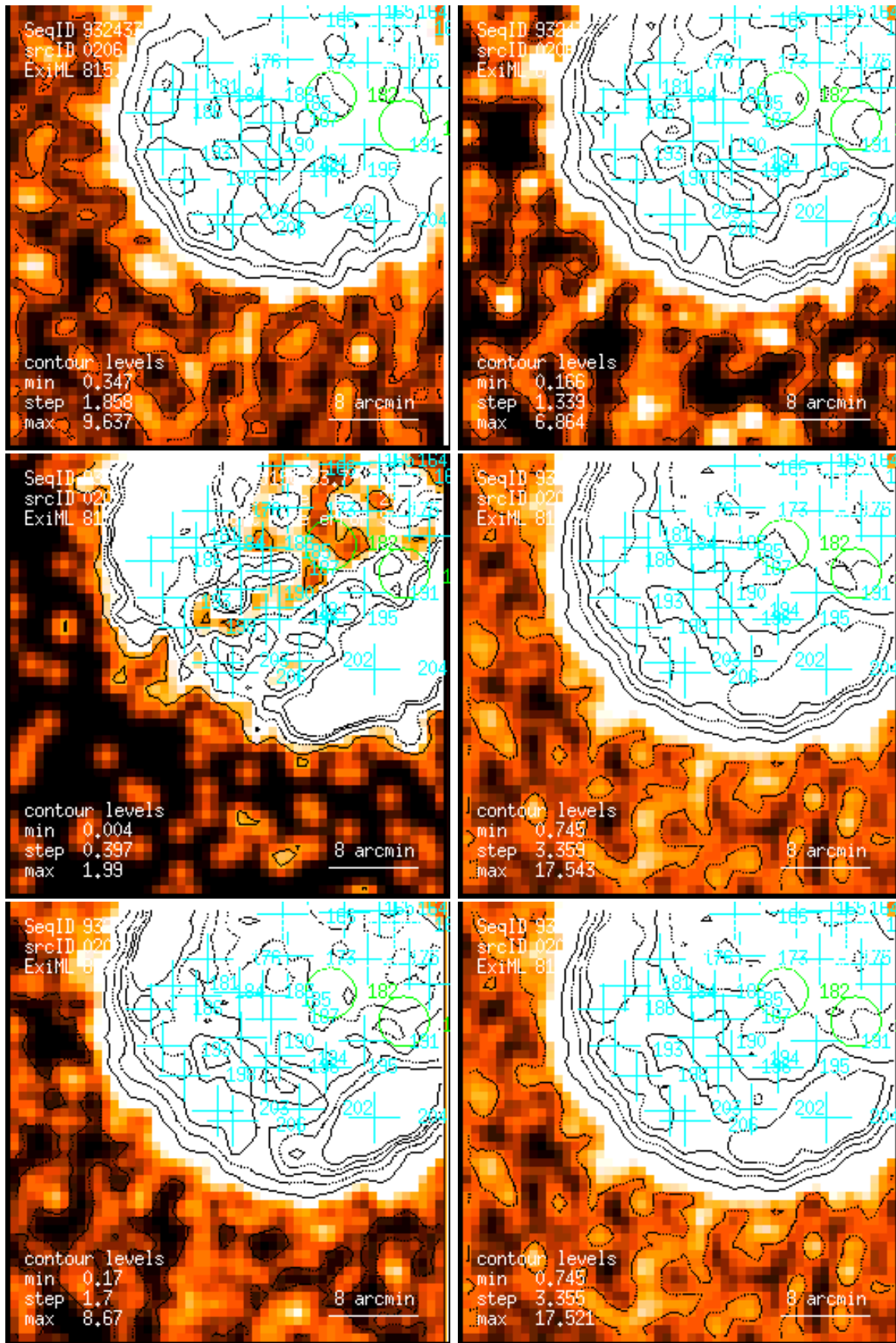
Figure 206: RASS 932433: detection 0206: band rate images, Gaussian filter: (1) PSPC channels 11 – 41, (2) 52 – 90, (3) 91 – 201, (4) 11 – 235, (5) 52 – 201, (6) 11 – 201. Broad band rates in counts/ks. Band rate contour levels in counts/ks/arcmin 2 .
