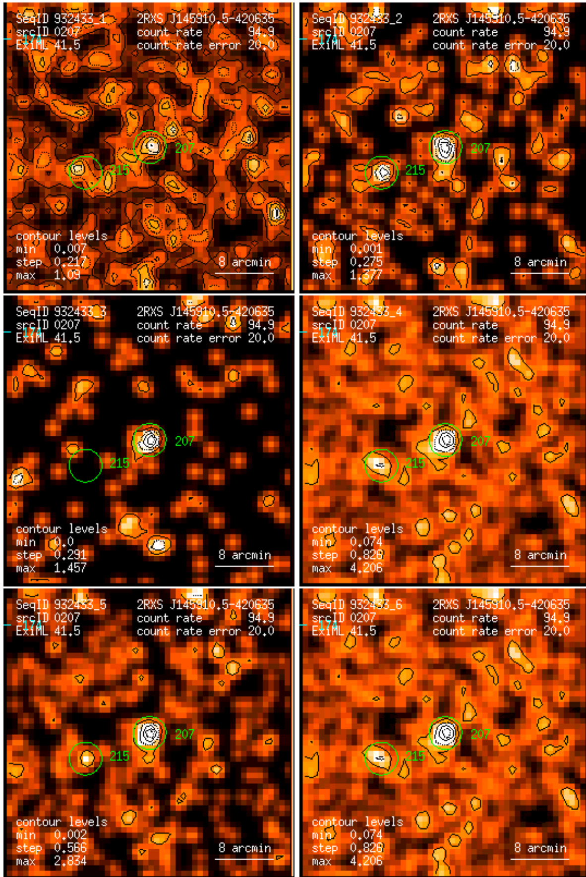
Figure 207: RASS 932433: detection 0207: band rate images, Gaussian filter: (1) PSPC channels 11 – 41, (2) 52 – 90, (3) 91 – 201, (4) 11 – 235, (5) 52 – 201, (6) 11 – 201. Broad band rates in counts/ks. Band rate contour levels in counts/ks/arcmin 2 .
