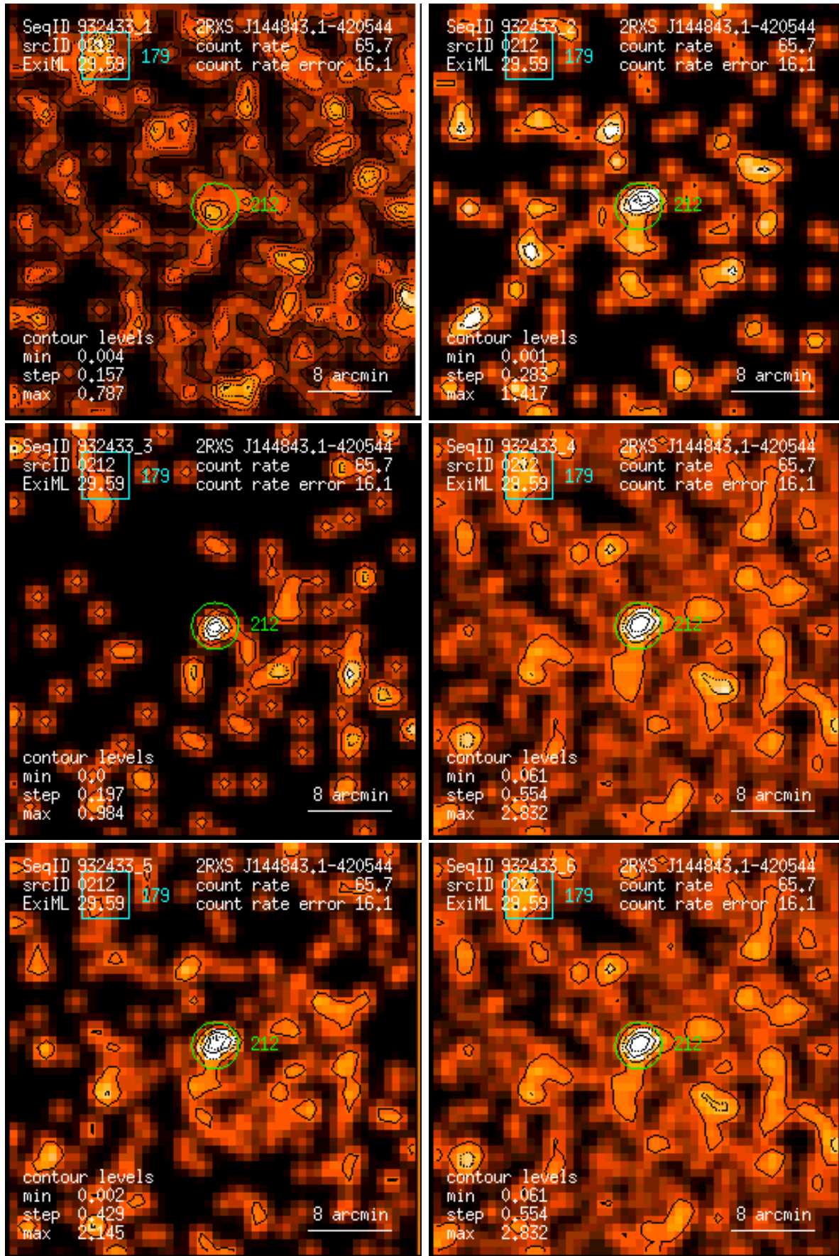
Figure 212: RASS 932433: detection 0212: band rate images, Gaussian filter: (1) PSPC channels 11 – 41, (2) 52 – 90, (3) 91 – 201, (4) 11 – 235, (5) 52 – 201, (6) 11 – 201. Broad band rates in counts/ks. Band rate contour levels in counts/ks/arcmin 2 .
