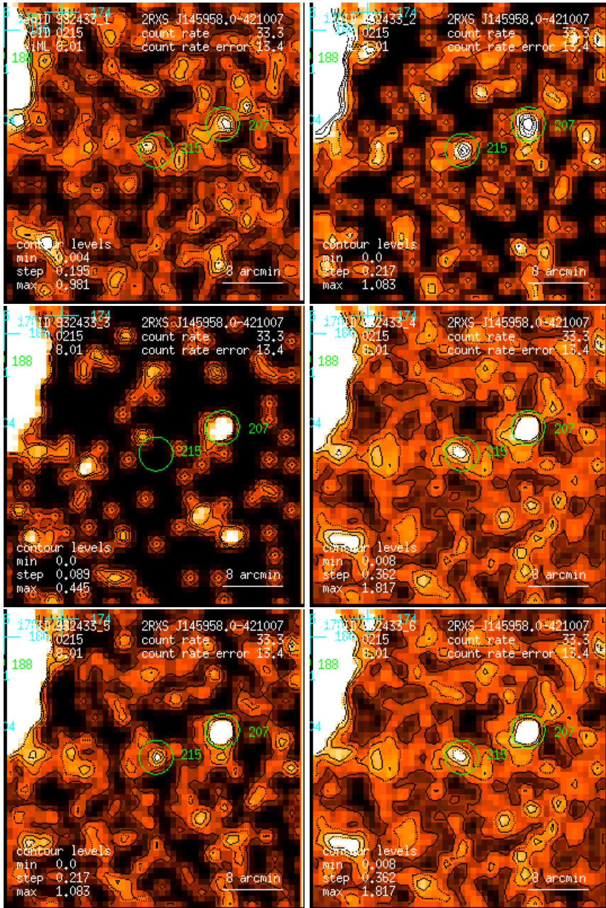
Figure 215: RASS 932433: detection 0215: band rate images, Gaussian filter: (1) PSPC channels 11 – 41, (2) 52 – 90, (3) 91 – 201, (4) 11 – 235, (5) 52 – 201, (6) 11 – 201. Broad band rates in counts/ks. Band rate contour levels in counts/ks/arcmin 2 .
