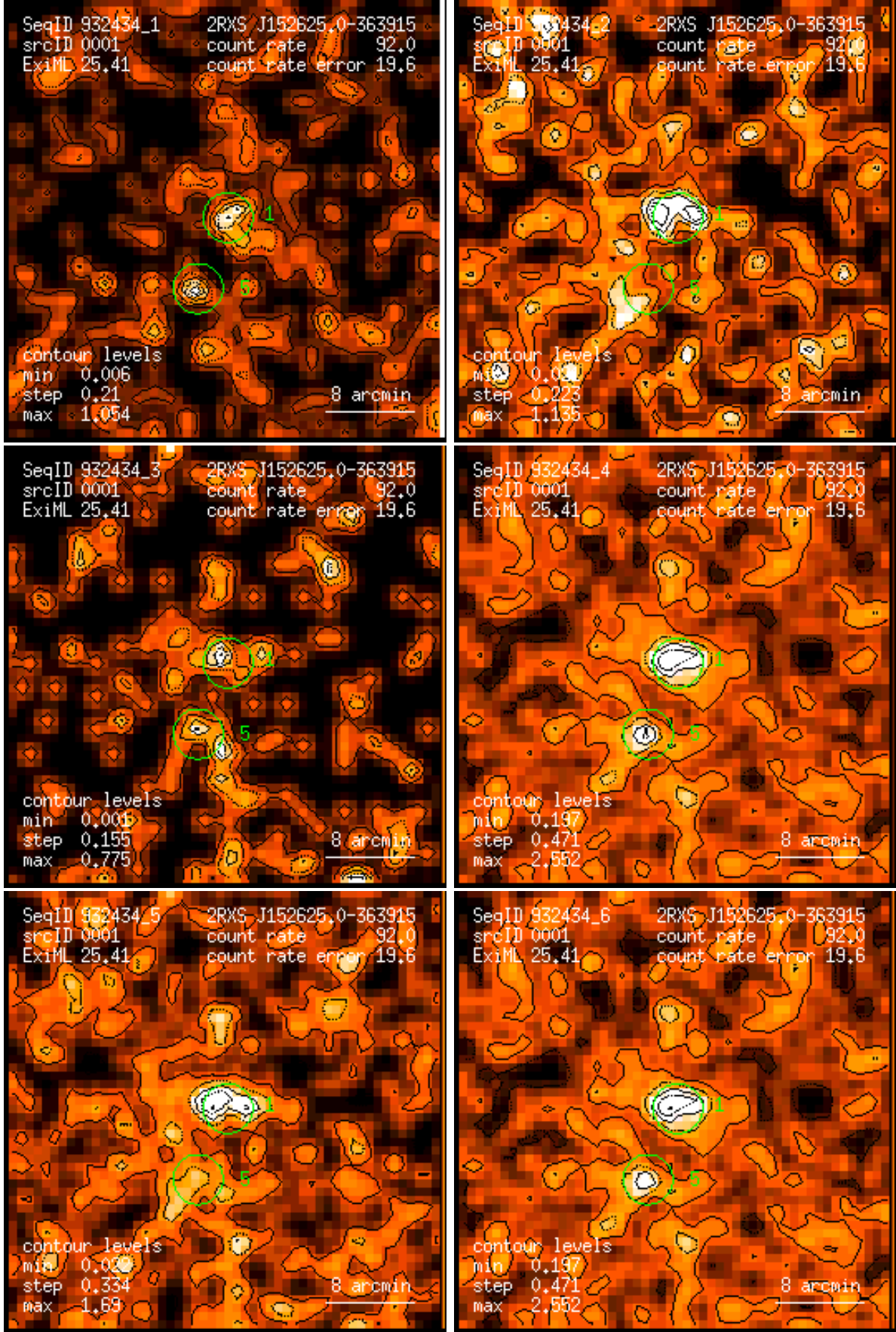
Figure 1: RASS 932434: detection 0001: band rate images, Gaussian filter: (1) PSPC channels 11 – 41, (2) 52 – 90, (3) 91 – 201, (4) 11 – 235, (5) 52 – 201, (6) 11 – 201. Broad band rates in counts/ks. Band rate contour levels in counts/ks/arcmin 2 .
