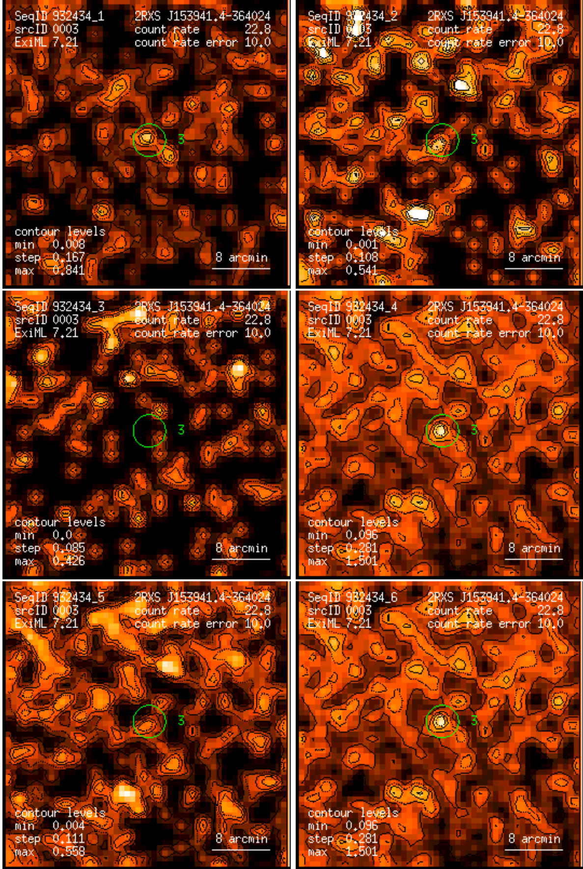
Figure 3: RASS 932434: detection 0003: band rate images, Gaussian filter: (1) PSPC channels 11 – 41, (2) 52 – 90, (3) 91 – 201, (4) 11 – 235, (5) 52 – 201, (6) 11 – 201. Broad band rates in counts/ks. Band rate contour levels in counts/ks/arcmin 2 .
