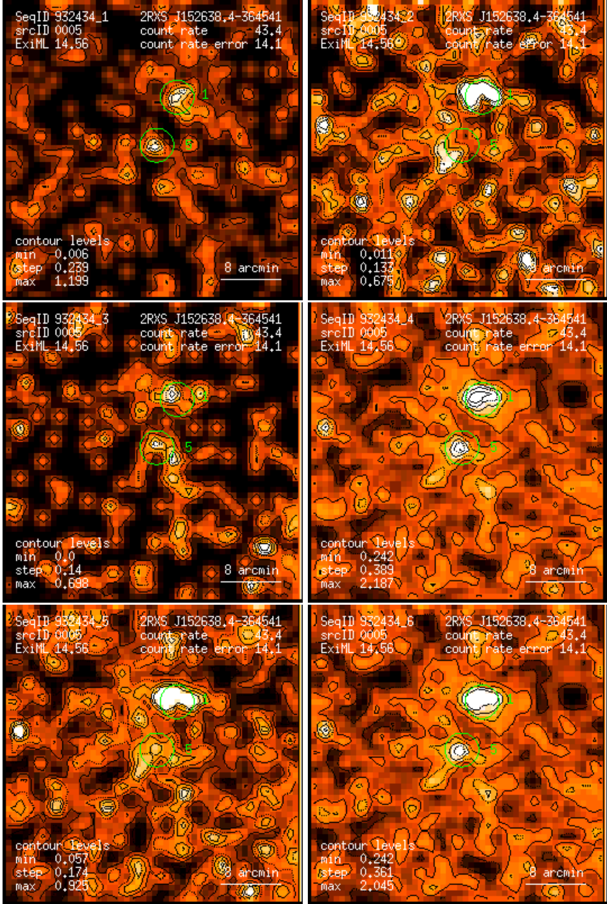
Figure 5: RASS 932434: detection 0005: band rate images, Gaussian filter: (1) PSPC channels 11 – 41, (2) 52 – 90, (3) 91 – 201, (4) 11 – 235, (5) 52 – 201, (6) 11 – 201. Broad band rates in counts/ks. Band rate contour levels in counts/ks/arcmin 2 .
